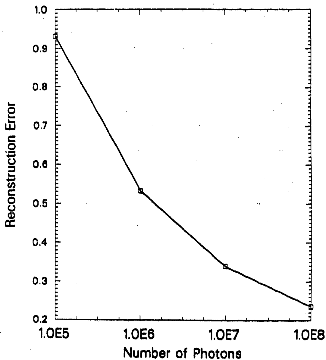
FIGURE 5-7. NORMALIZED RMS ERROR VS. NUMBER OF PHOTONS.
