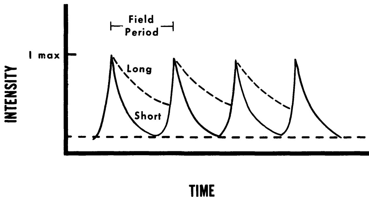
FIGURE 15. Interaction of a short persistence phosphor and a long persistence phosphor with the field rate period.
