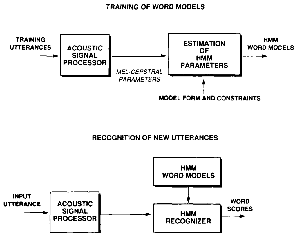
Figure 3-1. Baseline HMM isolated-word recognition system.
