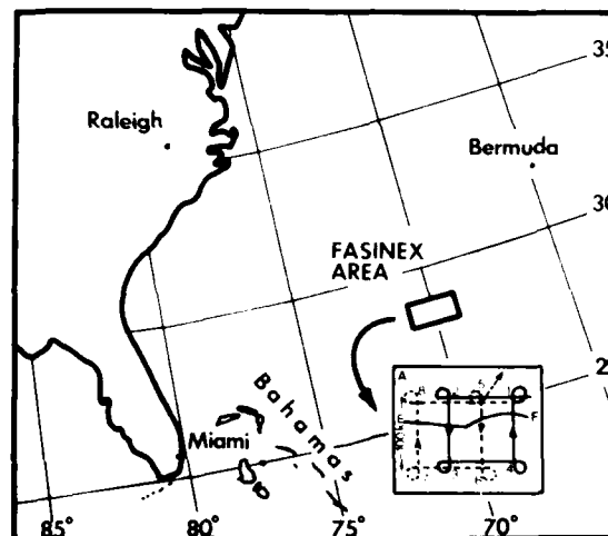
FIG. 1. Map showing the location of the FASINEX area. Aircraft were deployed from Raleigh, NC; Wallops Island, VA; Miami, FL and Bermuda. Insert A is a schematic of the turbulence aircraft flight pattern in the vicinity of the front (denoted by F).
