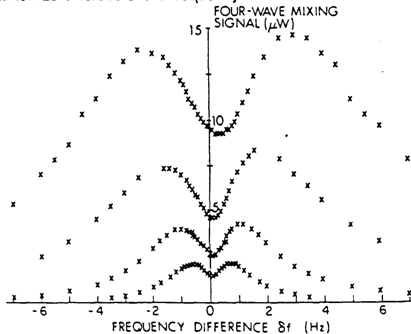
Figure 7. Measured efficiency for four-wave mixing vs. the frequency difference between the two writing beams in a photorefractive crystal of BaTiO_3 . The efficiency shows a marked increase when the frequency difference is non-zero, as predicted by the theoretical curve above.
