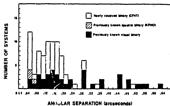
FIG. 1. The histogram of angular separations from 93 measurements of binary systems clearly shows the increase in newly resolved systems at separations less than 0.25 arcsec. An additional 22 measures of systems with separations exceeding 0.65 arcsec are not shown here. Those "wide" binaries include only one newly resolved system.
