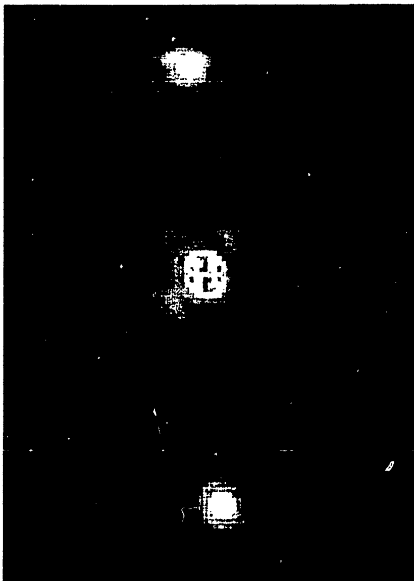
Figure 3. The binary star ADS 7158 has an angular separation of 0.24 sec, so close that the speckle patterns of the two component stars cover each other in an image taken with the Kitt Peak 4-m telescope (top). A vector-autocorrelogram (bottom) gives an accurate measure of the angular separation and relative orientation of the two stars. The two outer peaks in this computer-generated image represent the paired speckles in nearly 2,000 individual speckle frames like the one at the top. The bright central peak results from the superimposition of every speckle.
