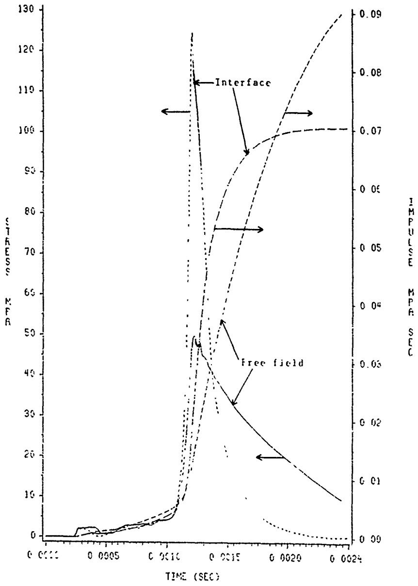
Figure 15. Comparison of Pressure and Impulse Histories at Center of Concrete Slab between Free-Field and 150 cm Standoff Distance Calculations.
