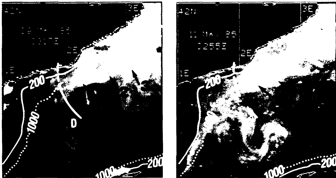
Fig. 7. Thermal features advecting within the Catalan Front (cold water plume). The features indicated by the arrows moved at approximately 20 cm/s and continued into the filament associated with submarine canyon D. During the period May 1–13, the movement of several similar thermal features could be monitored from image to image. During this time, features in the warm water outside the plume and filament showed comparatively little movement. The filament did show some later displacement. However, this movement was much less than the speed of the thermal features inside the filament.
