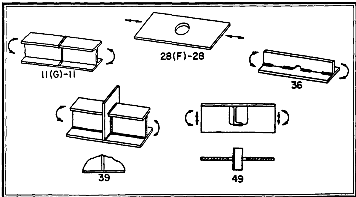
Figure 3-6. Local Fatigue Details for the Cape-Class (Munse, 1982)
