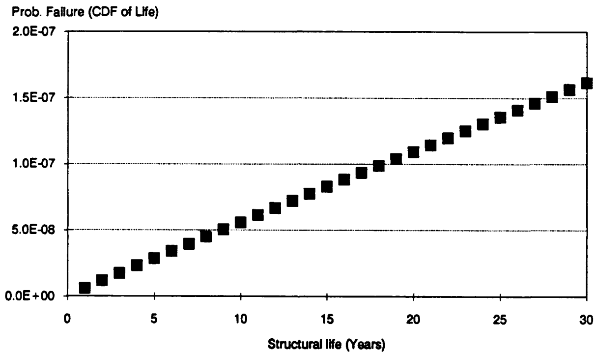
Figure 5-9. Structural Life Based on Fatigue Failure for the Example Case
