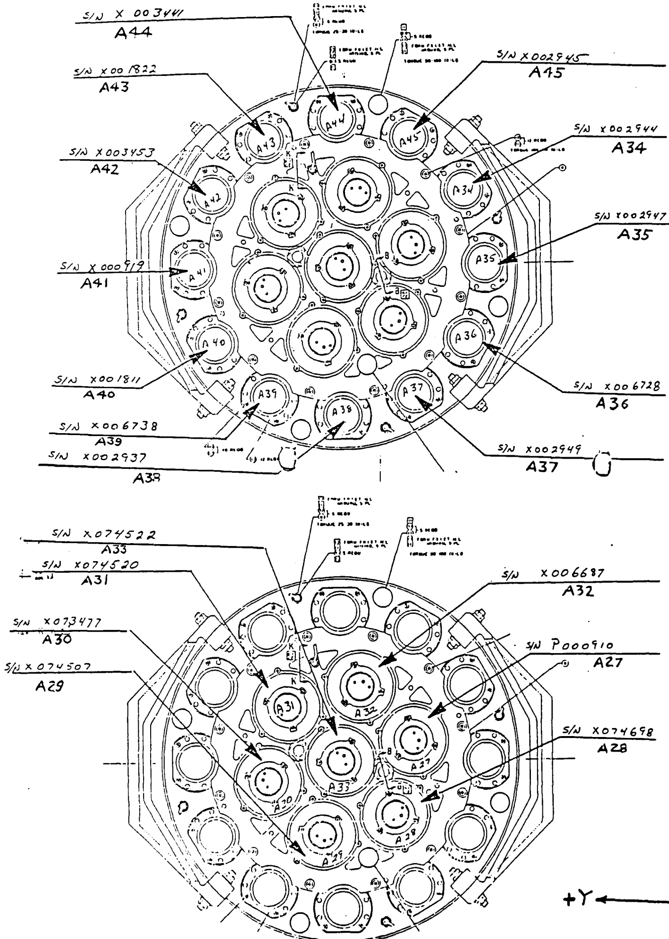
FIGURE 2-2. DETECTOR A2 PMT IDENTIFICATION
