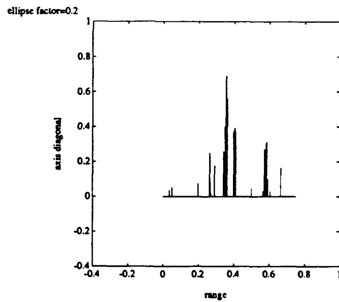
Figure 4.29: 747 Scatterers and Polarizations, SNR of 0dB
