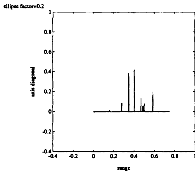
Figure 4.27: 747 Scatterers and Polarizations, SNR of 10dB
