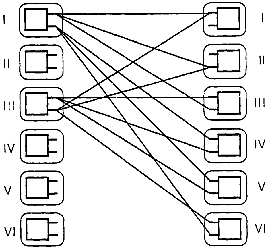
Fig. 2.21 Interconnection for 1.5C^2 with C_T = C_R , both even. Each group is represented by a single station, and the interconnection is shown for TS groups I and III. ( C = 2 .)
