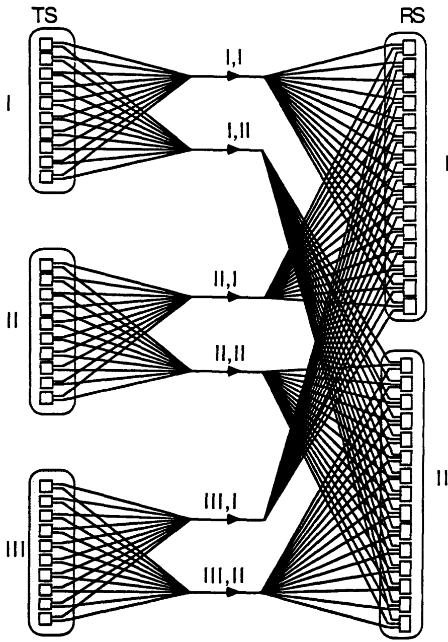
Fig. 2.10 Single-path, unidirectional, equal-degree SBI with disjoint subnetworks and grouping; C_T \neq C_R . ( N = 30 ; C_T = 2 ; C_R = 3 .)
