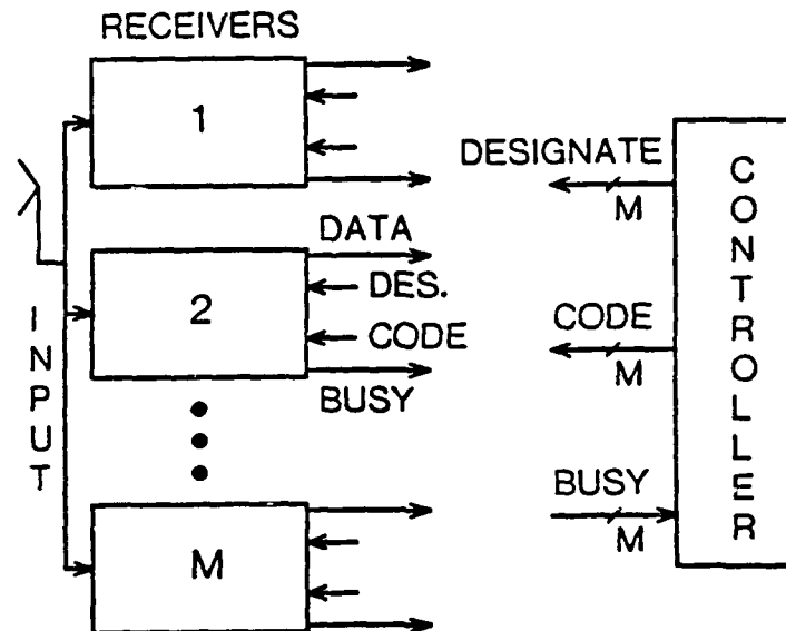
Fig. 4.17 Dynamic-code-assignment architectures. (DCAA.)
