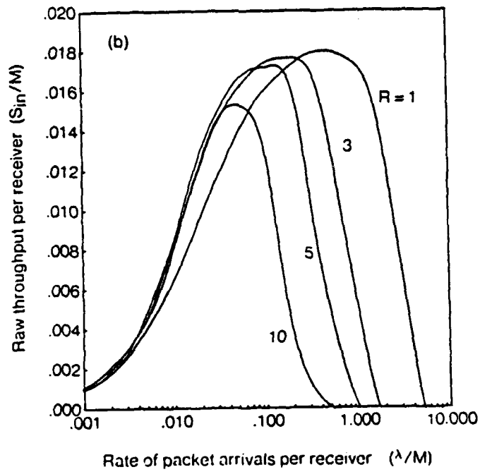
Fig. 4.15 Inbound throughput per receiver with FCAA for various group sizes. a) \frac{1}{\mu} = 10 ; b) \frac{1}{\mu} = 50 .
