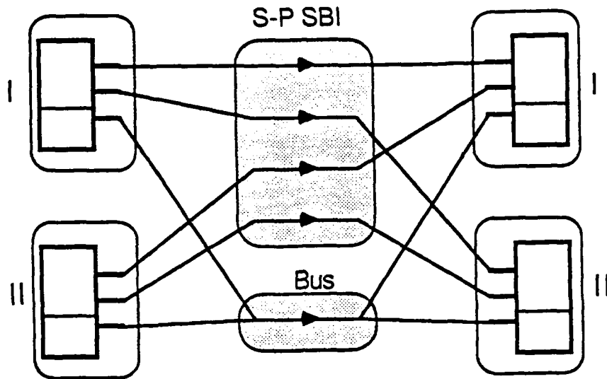
Fig. 2.13 Unidirectional hybrid SBI-PBI . C = 3 , C' = 1 .
