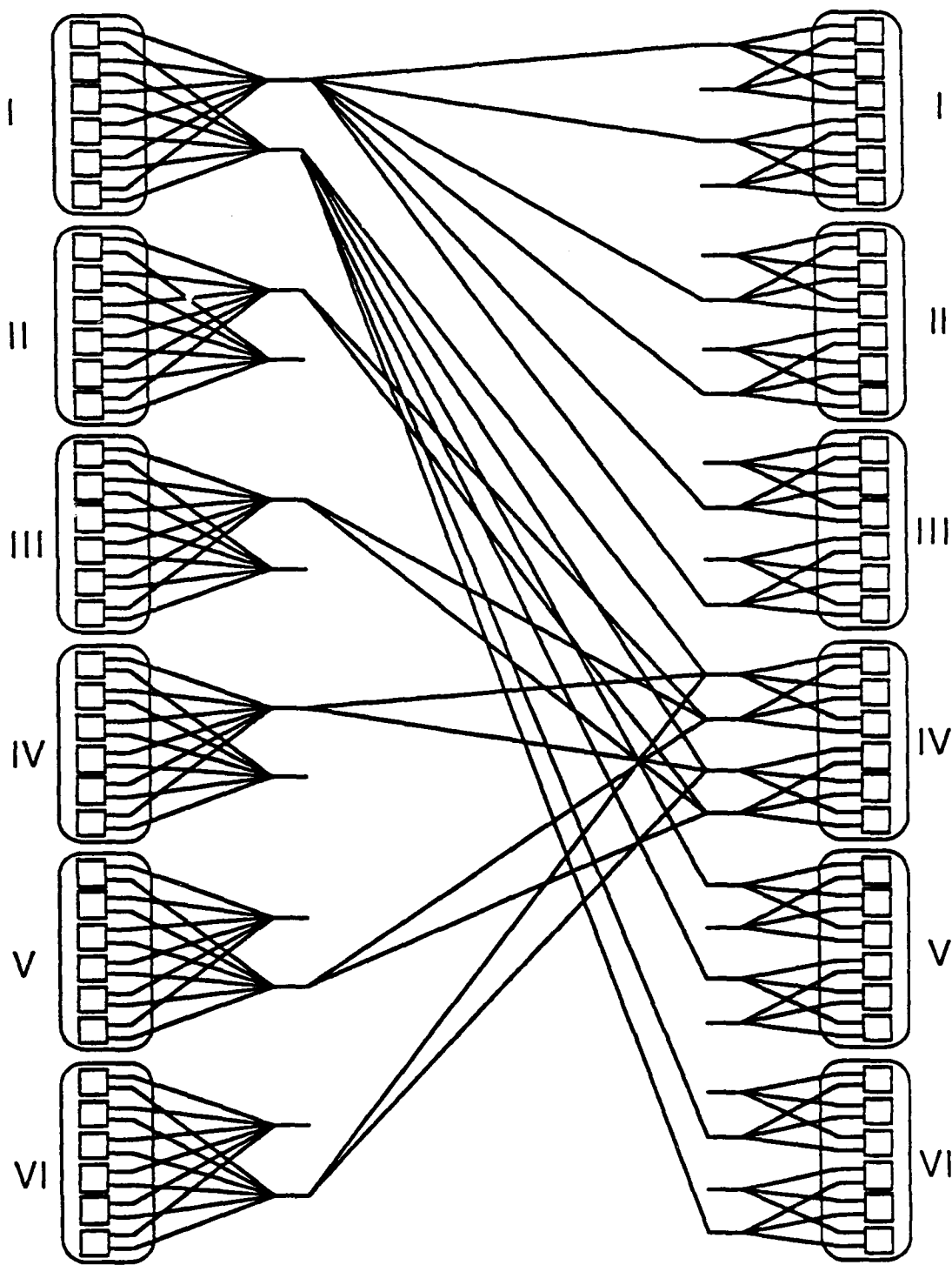
Fig. 3.3 Power-efficient fiber optic configuration for the SBT that achieves 1.5 \cdot C^2 with a uniform traffic pattern. The connections are shown for the 1st TS group and for the 4th RS group.
