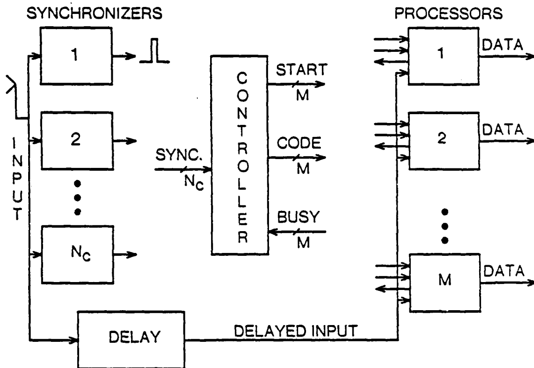
Fig. 4.18 Causal implementations of the seemingly noncausal DCAA-OA. The figure shows the pipelined version; the non pipelined version is obtained by removing the "start" signals and replacing "processors" with "receivers."
