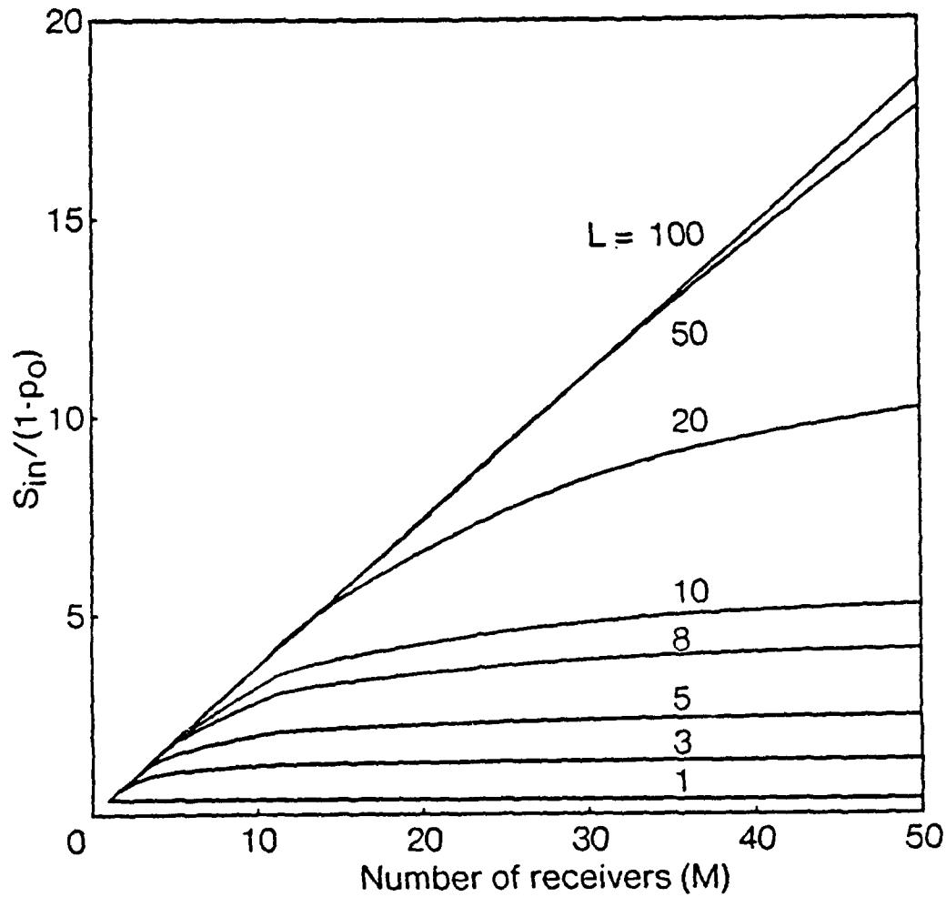
Fig. 4.4 Maximum normalized inbound throughput with multiple receivers. (Slotted). N = 100 ; p \approx p_{opt}(N, M, L) .
