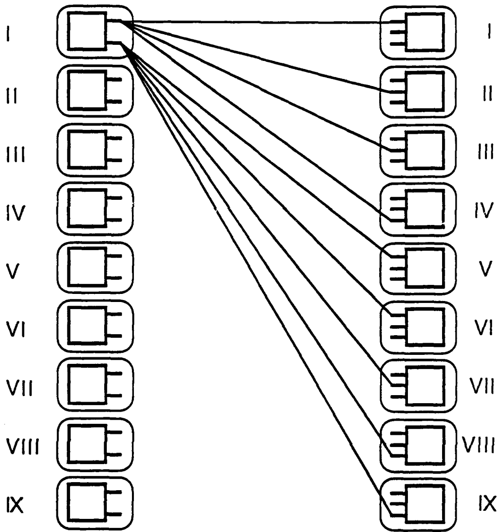
Fig. 2.23 Interconnection for 1.3C_T C_R with C_T \neq C_R ; C_T is even, but C_R is odd. Each group is represented by a single station, and the interconnection is shown for a single group of TS's. ( C_T = 2 , C_R = 3 .)
