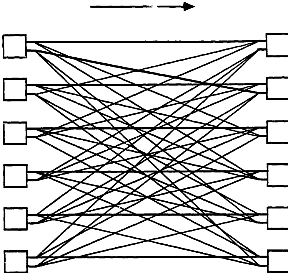
Fig. 2.25 An equal-degree SBI which achieves the upper bound on concurrency. The thick edges are mutually noninterfering. N = 6 ; C = 2 ; maximum concurrency = 7.
