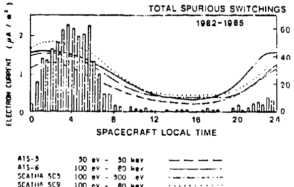
Fig 6. Diurnal spread of MARECS-A spurious switchings compared with average profiles of measured currents.
