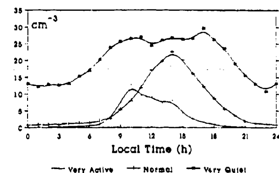
Fig 5. Diurnal variation of mean cold plasma concentration at GEO for 3 levels of geomagnetic activity: GEOS-2, 1978-80.
