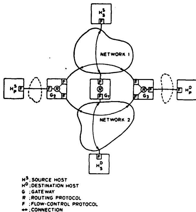
Fig. 4 Example of a network interconnection.
