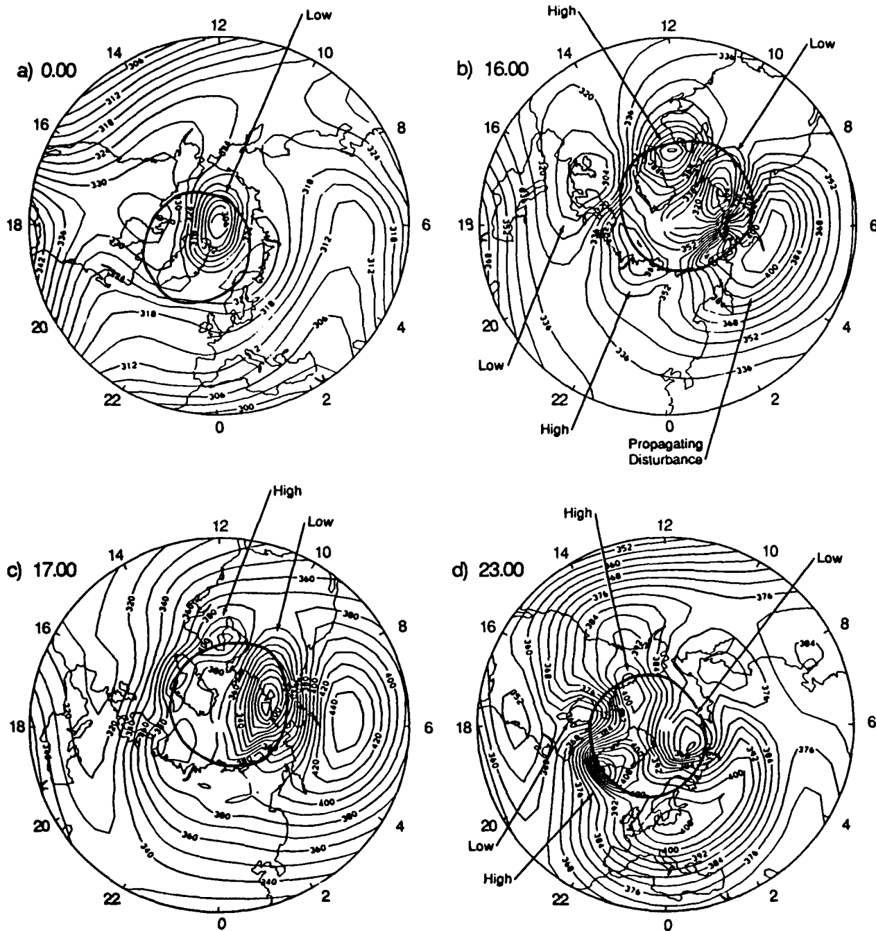
Fig. 17. Development of total mass density ( \times 10^{-15} \text{ g cm}^{-3} ) at 200 km for the northern hemisphere ( 30^\circ\text{--}90^\circ\text{N} ) during the TGCM simulation of September 19, 1984: (a) 00 UT, (b) 16 UT, (c) 17 UT, and (d) 23 UT. The main high- and low-density features are labeled appropriately.
