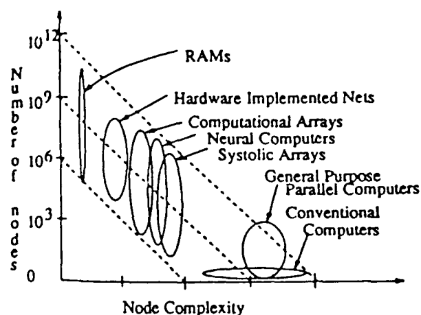
Figure 14. Spectrum of neurocomputer architectures.
