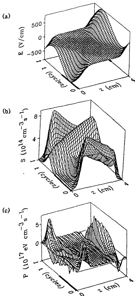
FIG. 1. Benchmark run: (a) electric field E(z,t) , (b) primary ionization rate per unit volume S(z,t) , and (c) power deposition into the electrons P(z,t) = -n_e |e| E_z(v_r) , over one rf cycle T = 7.375 \times 10^{-8} s. The heavy portions of the z=0 and z=4 cm lines indicate parts of the rf cycle where the corresponding electrode is cathodic.
