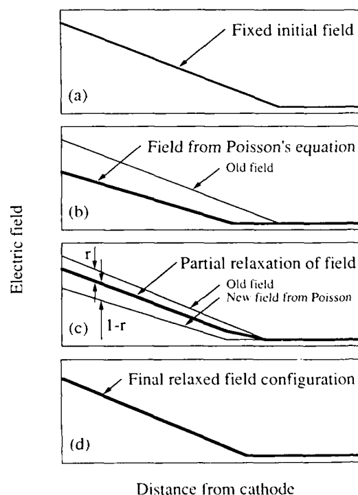
FIG. 6. Schematic of the field relaxation algorithm. Initial fixed-field configuration is guessed and the convective-scheme run to (near) stability (a). Poisson's equation is used to calculate a new field configuration (b). Old field is then allowed to relax a fraction r of the distance toward the new field (c). Partially relaxed field of (c) becomes the "old" field in (b) during the next iteration, and (b) and (c) are repeated until stability is again reached (d). Separation of the old and new fields, as well as the amount of relaxation r , have been exaggerated for clarity.
