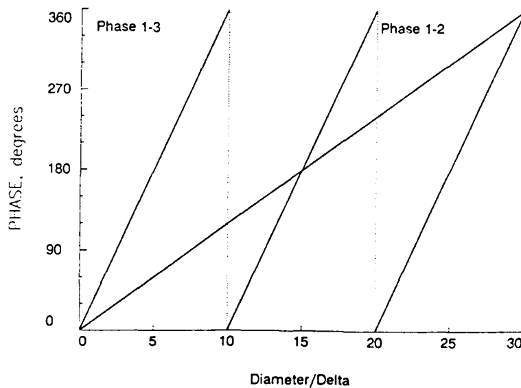
Figure 4. PDPA instrument response curves.
