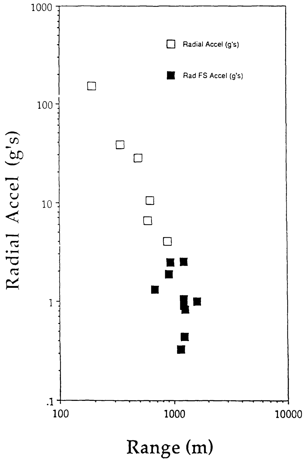
Figure 6 Free-field (open squares) and free surface (closed squares) peak radial accelerations from MISTY ECHO.
