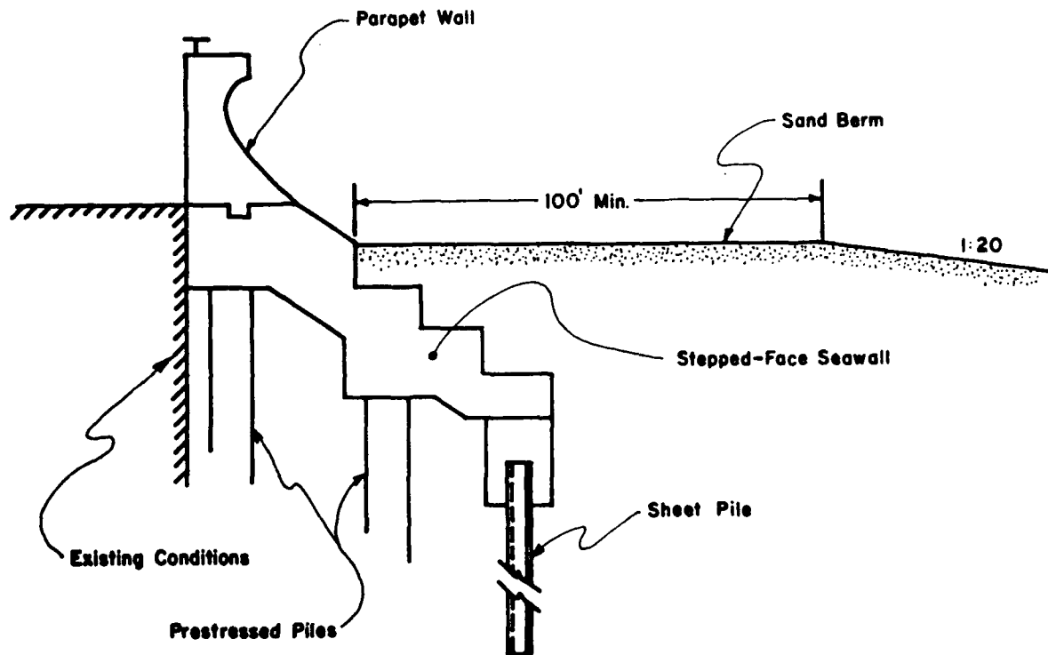
Figure 4. Typical design cross section with protective seawall with 100-ft-wide berm
