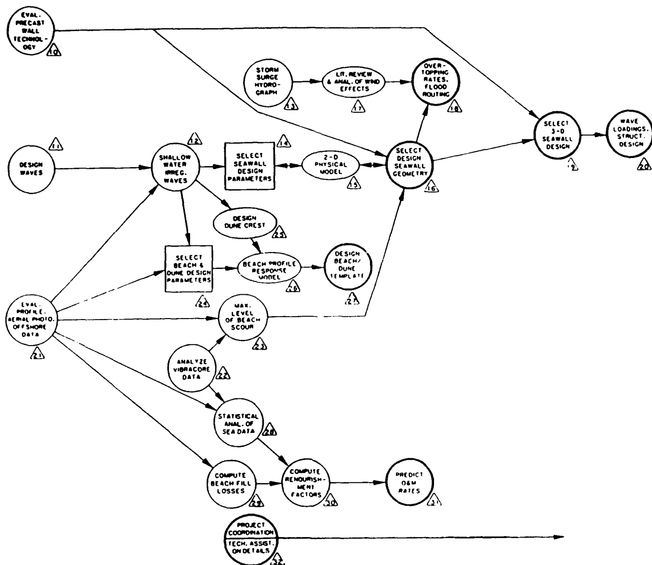
Figure 3. Flowchart for coastal engineering studies Virginia Beach, Virginia
