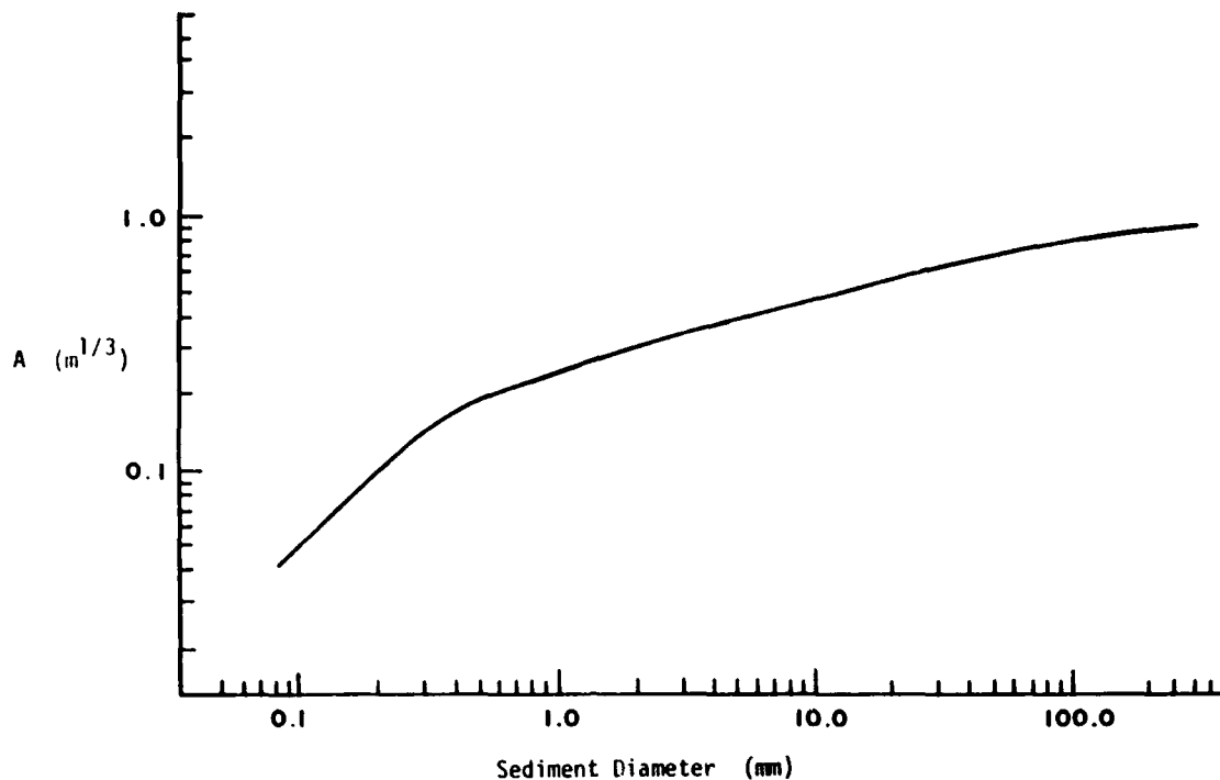
Figure 6. A versus sediment diameter (after Moore 1982)
