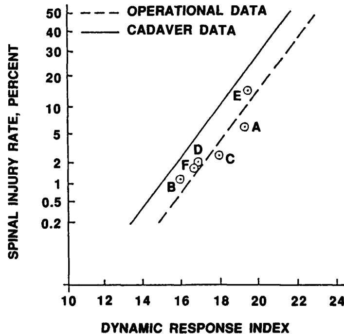
FIG. 5: CORRELATION BETWEEN DYNAMIC RESPONSE INDEX AND SPINAL INJURY RATE FOR EJECTION SEATS [REF. 26]
