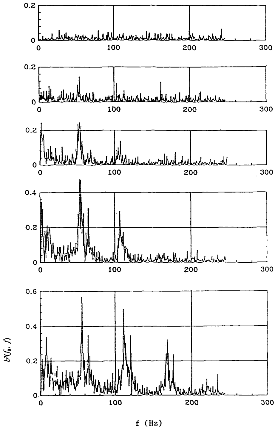
Figure 31 b^2(v_0, f) of the temperature disturbance at x/H = 2.5 y/H = 0.87 . Jet with q = 1.26 \text{ mm}^2/\text{s} and, from bottom to top, S = 0.77 , 0.86 , 0.87 , 0.89 and 0.92 .
