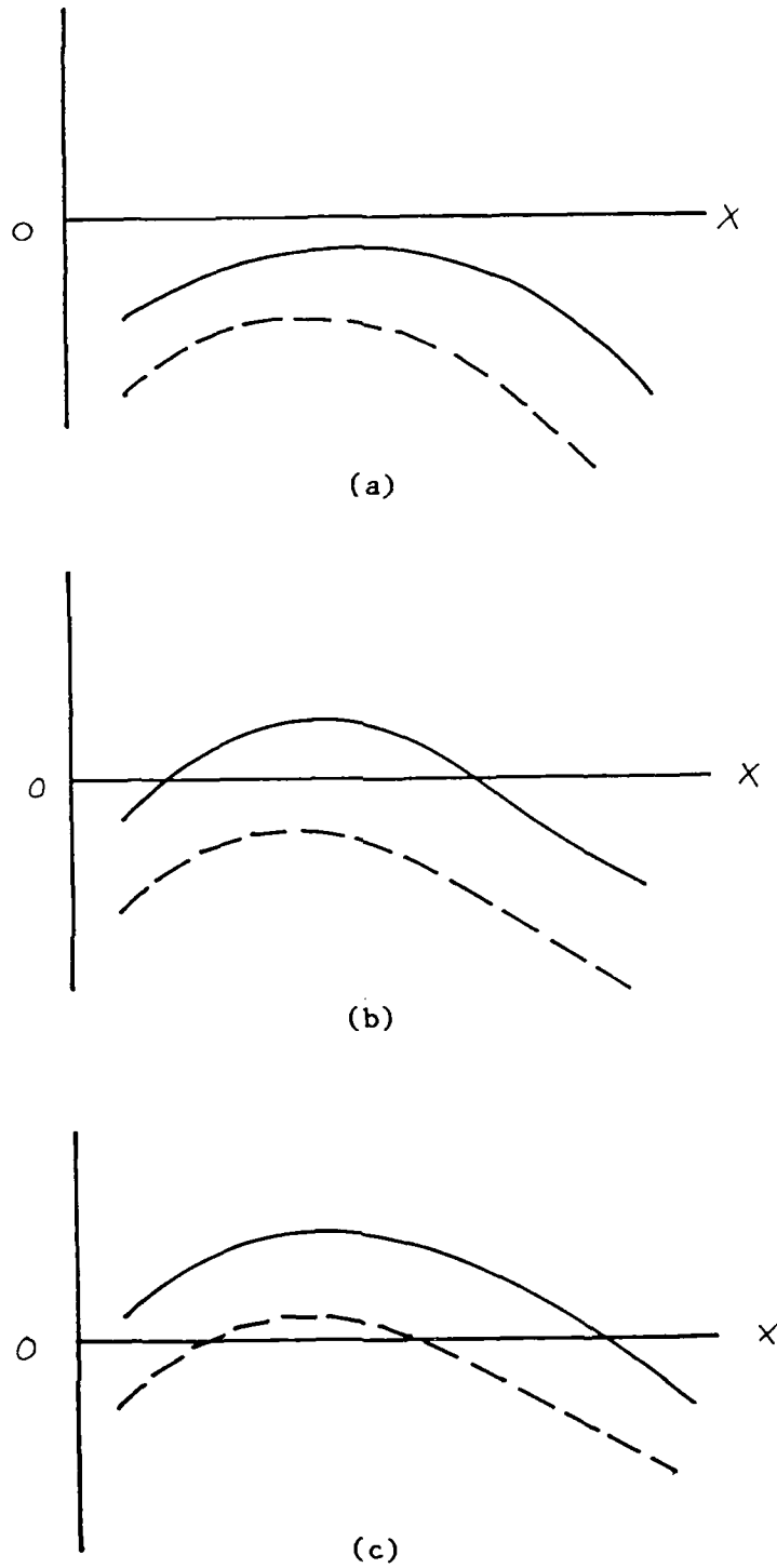
Figure 3 Sketch of the typical x -dependence of the local maximum temporal growth rate \omega_{max}^{\sigma} (—) and the local absolute growth rate \omega_a^{\sigma} (-----) in free shear flows for the case of: (a) uniform local stability; (b) local convective instability; (c) local absolute instability.
