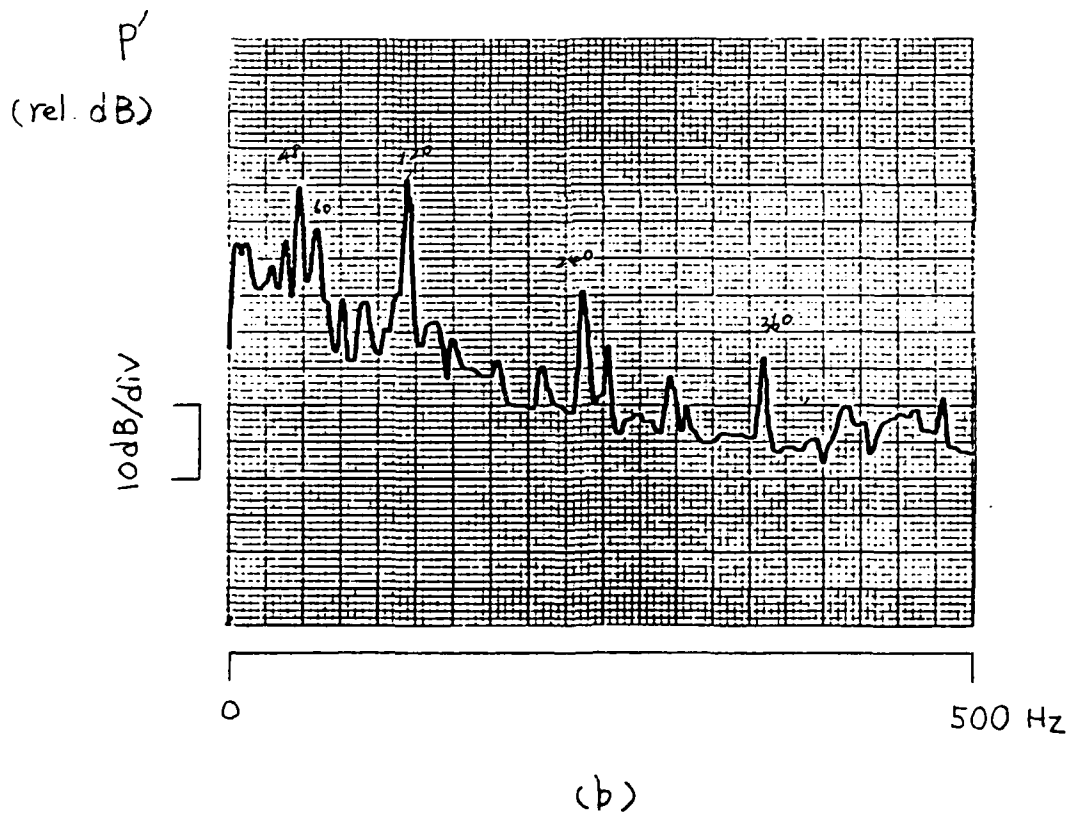
Figure 10 (a) The level of turbulent intensity of the 2-D jet facility at x=y=z=0 for q=1.25\text{ mmH}_2\text{O} , and (b) the acoustic pressure spectrum of the background noise with the jet turned off (microphone at x/H \sim 2 , y/H \sim 1.3 )
