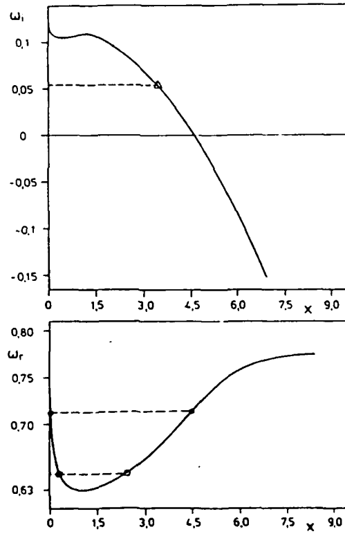
Figure 2 Local and global stability calculations by Hannemann (1988) for wake flow, (a) numerical simulation of wake flow used to calculate stability characters, (b) the growth rate \omega_i and frequency \omega_r , calculated by local linear theory (—) and global simulation (-----). \circ global frequency in nonlinear state, \square global frequency in linear regime.
