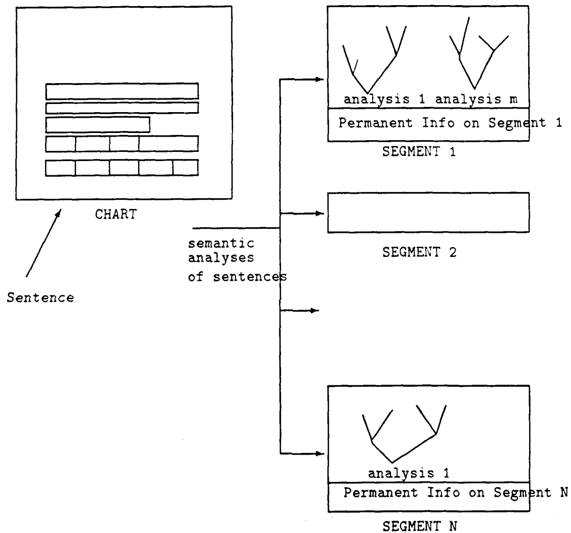
Figure 4.1: Architecture of the BlackBoard
