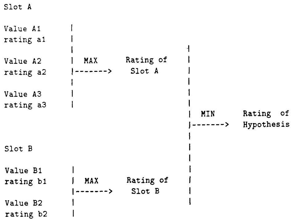
Figure 4.2: Computation of Ratings
