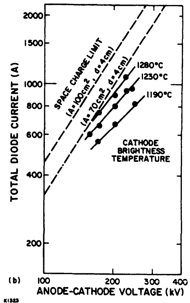
Figure IV-22 Voltage and Current Characteristics Measured for a 100 cm 2 Dispenser Cathode ( d_{ak} = 4 \text{ cm} ) a) \sim 10^{-6} torr b) \sim 10^{-7} torr
