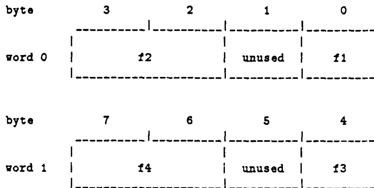
Figure 4. Pragma Pack Ignored
