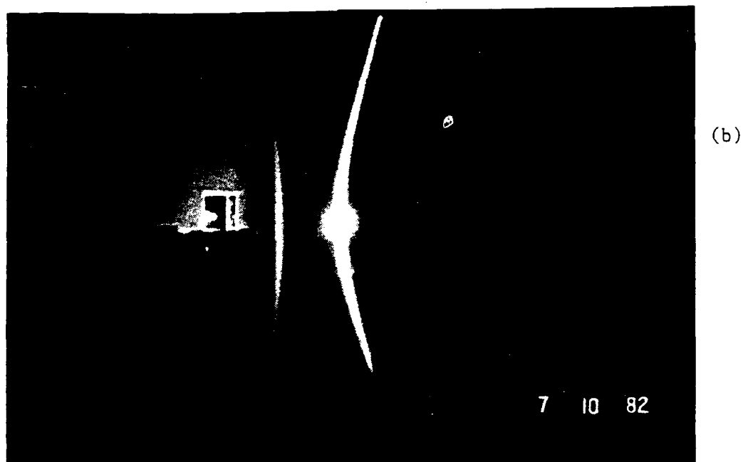
Figure 3.15. Photographs of the illumination of a screen by the light reflected from the films at resonance. The electromagnetic wave is scattered mainly in the dielectric layer of Fig. 3.14 and emerges as part of a cone of light.
