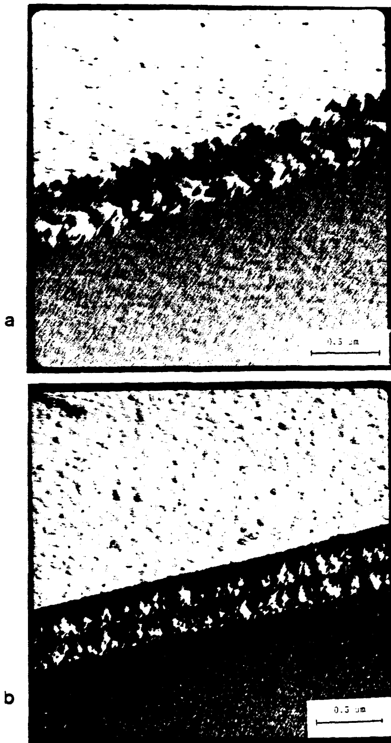
Figure 5.27. Micrograph (TEM) of thin-film multilayer of ZrO_2 (H) and SiO_2 (L). Lower half of photograph is glass.
