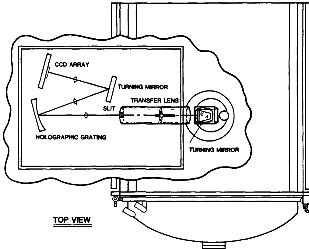
Fig. 2. Balzers 760 with scanning monochromator modification.
