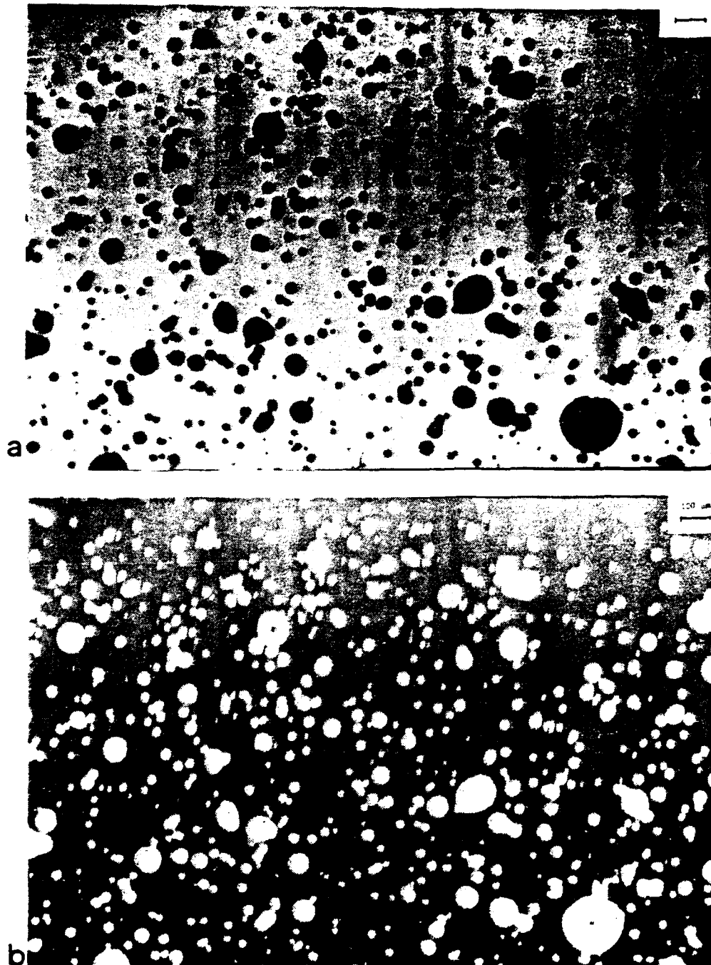
Figure 4.14. Water adsorption in Ag/Na 3 AlF 6 filter. Sample ML-11-6, set in RH = 75% for 5 hr. (a) \lambda = 543 nm. (b) \lambda = 547 nm.
