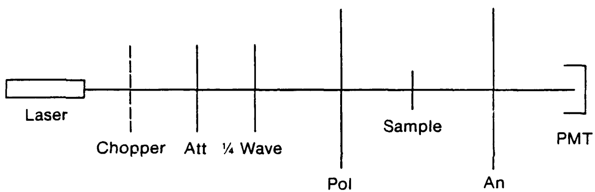
Figure 2.1. Characterization Setup.
