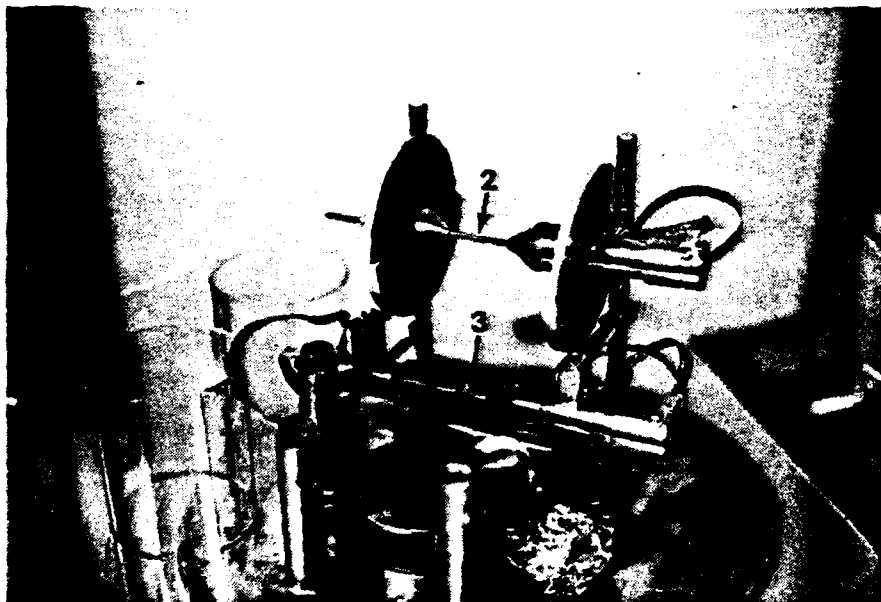
Figure 2.3. Two-inch coating unit for making TEM replicas.
