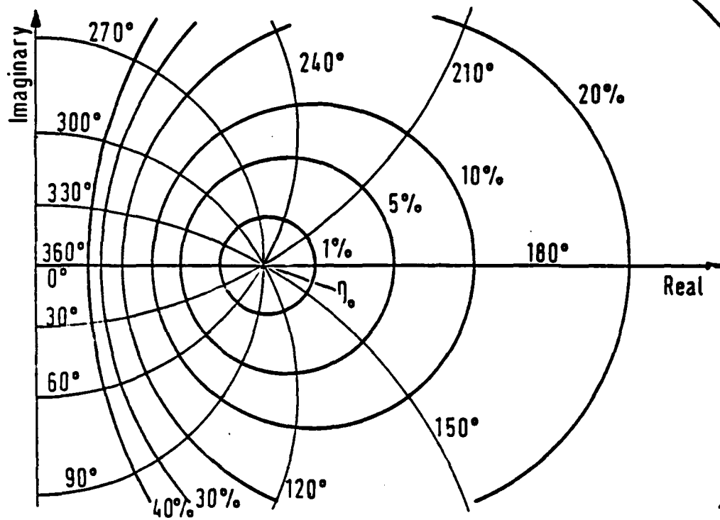
Figure 3.2. Isorefectance and isophase contours (Macleod, 1980).
