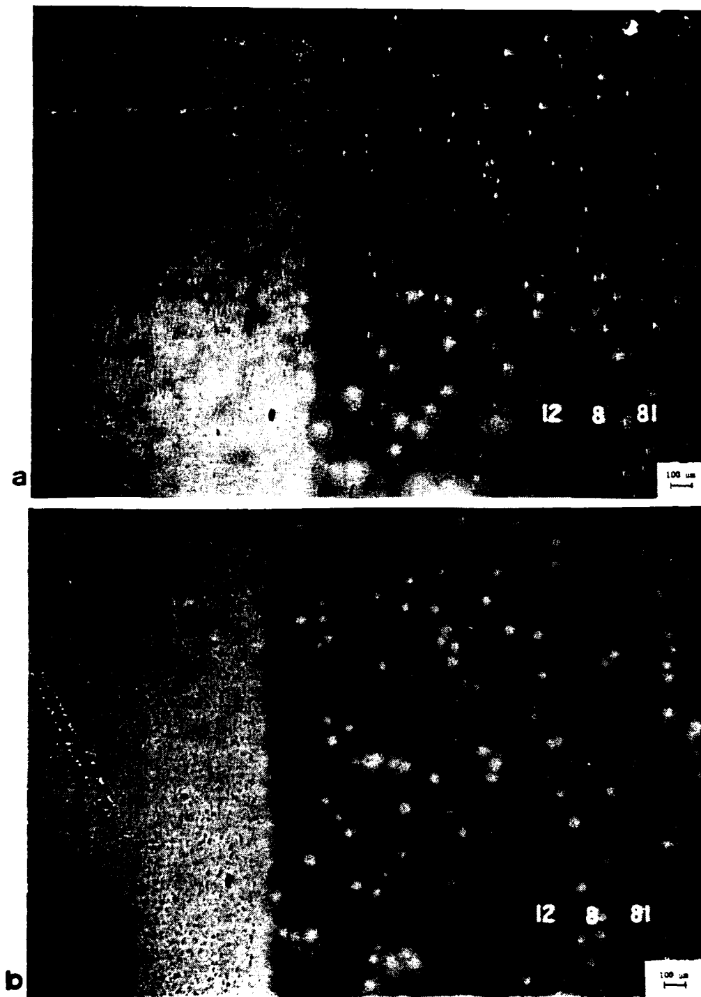
Figure 6.3. Water adsorption in ZnS/ \text{AlF}_6 filter. Left side of photographs is with sandblasted substrate and right side is without sandblasting. (a) After 50 minutes, (b) after 150 minutes.
