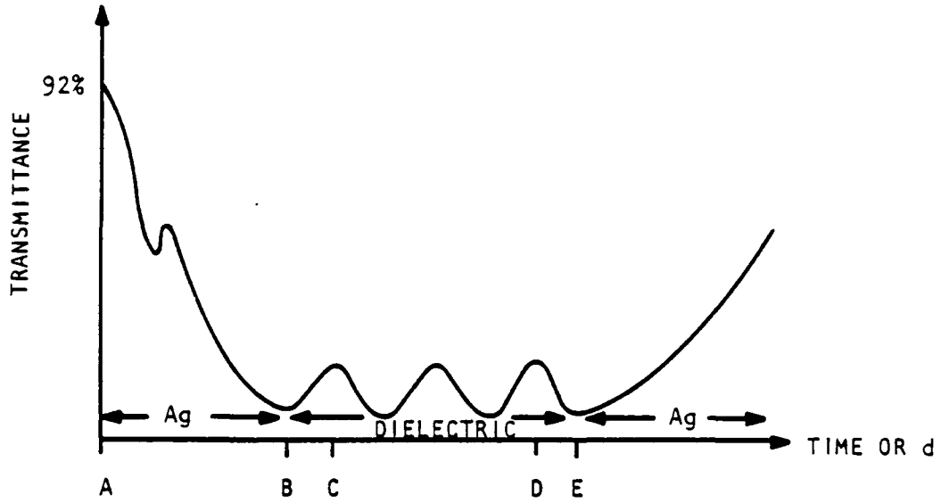
Figure 4.2. Measurement of transmittance of a growing filter.
