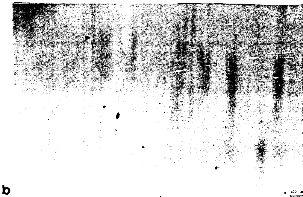
Figure 5.31. Water adsorbed filters after baking. Sample 760-17-3 after baking at 370^{\circ}\text{C} for 1.5 hr in vacuum. The patches disappeared and reappeared when exposed to air. \Delta\lambda_{ad} = 50\text{\AA} , \Delta\lambda_{bk} = -25\text{\AA} . (a) \lambda = 544.5\text{ nm} . (b) \lambda = 550.5\text{ nm} .
