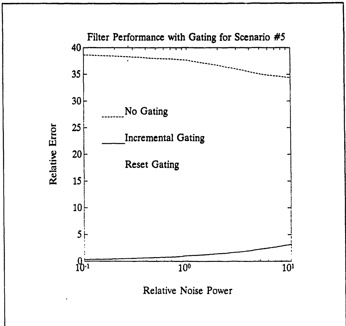
Figure 7.11: Filter Performance for Scenario #5
