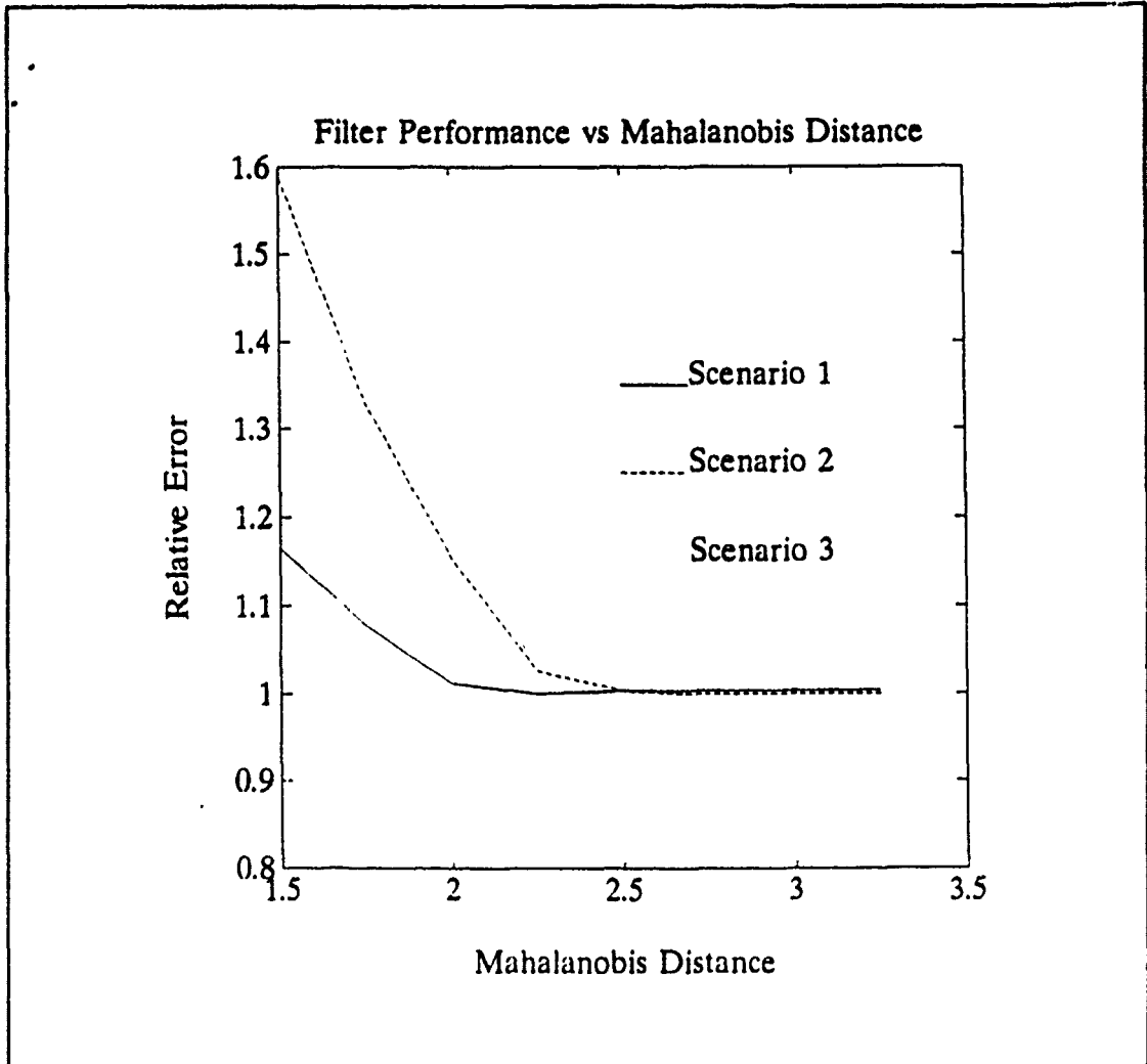
Figure 7.6: Filter Performance as a Function of Gate Size for Non-Maneuvering Targets
