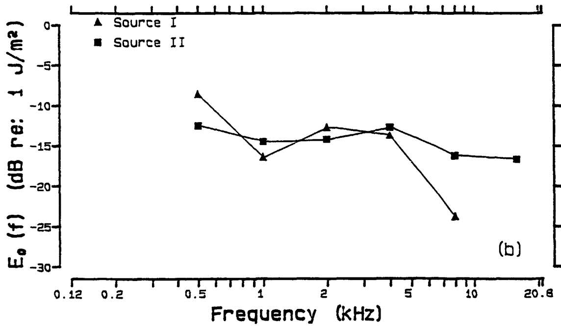
Figure 17. (a) The slope of the regression line relating PTS_{90} and the exposure energy level across the range of audiometric test frequencies for the two impulse noise sources. (b) The threshold energy level E_0(f) at each audiometric test frequency and for each impulse source for which 90 percent of the exposed population will not sustain a PTS.
