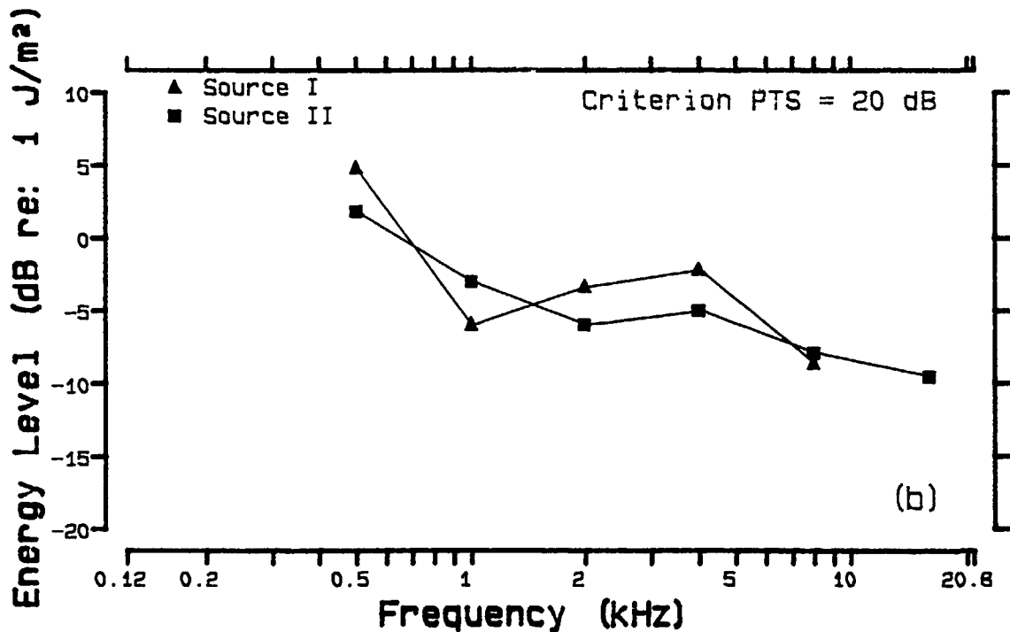
Figure 18. (a) The PTS 90 that can be expected at each audiometric test frequency for an impulse having a 1 J/m 2 energy flux in each of the octave bands centered on the audiometric test frequencies. (b) The energy level in the octave band centered at each audiometric test frequency that will produce a criterion PTS 90 of 20 dB.
