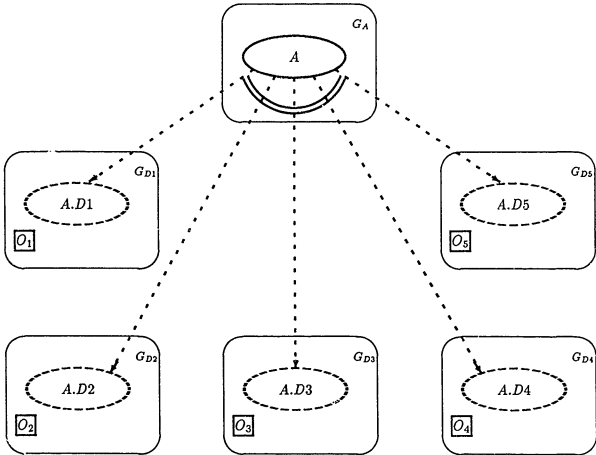
Figure 6-1: The replication example: Up to 2 sites can be ignored during Two Phase Commit.
