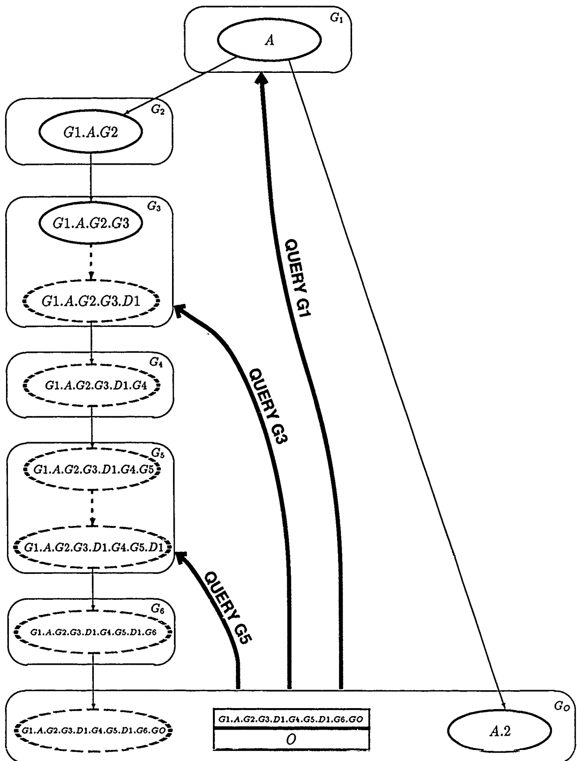
Figure 3-2: An example for a site making queries about the fate of a lock owner.
