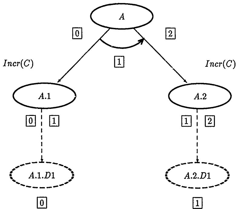
Figure 4-3: An action tree, with timestamps, for the action A that updated the counter C twice using serial subactions.
