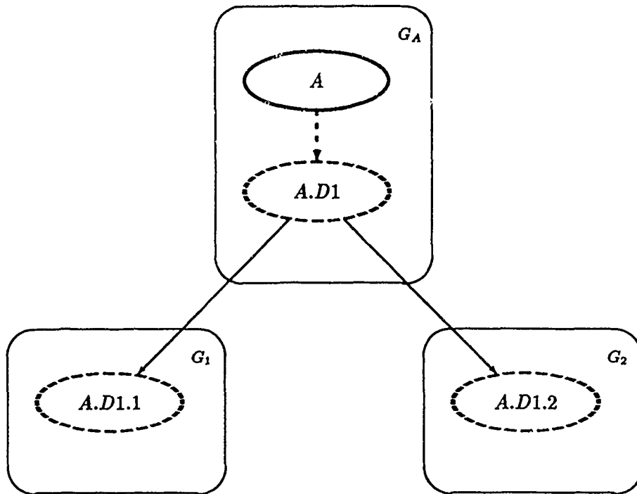
Figure 3-1: An example of a Disconnected Action
