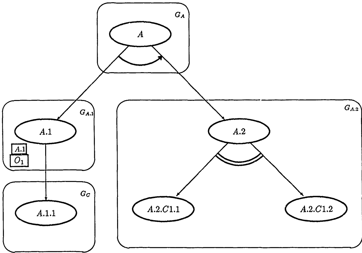
Figure 2-3: An example for an action tree.
