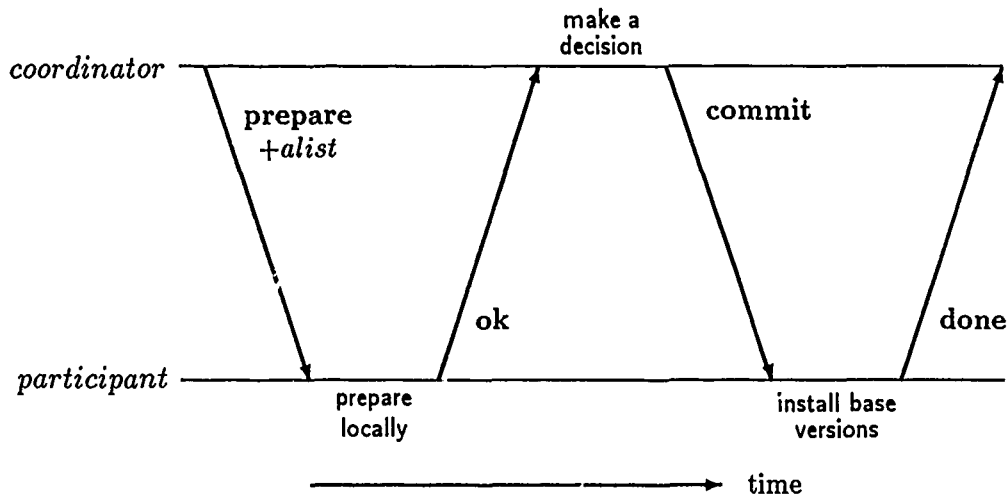
Figure 2-4: A time-space diagram of the current Two Phase Commit protocol.
