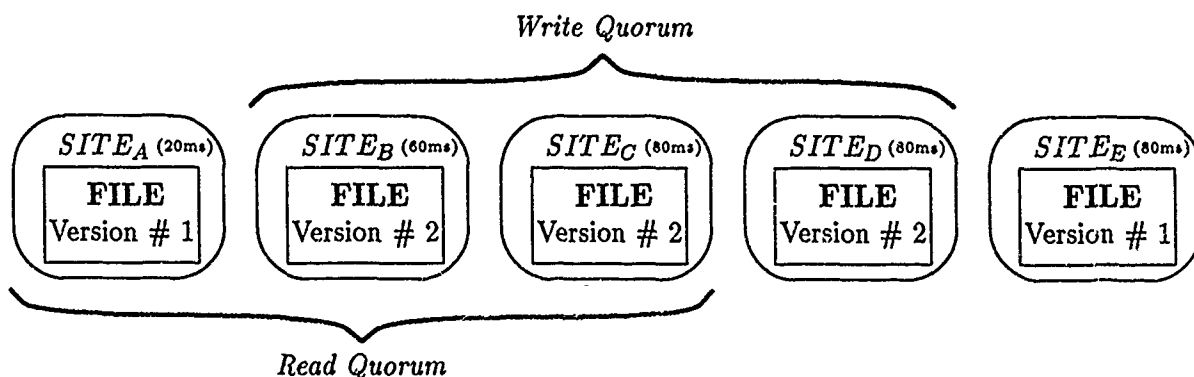
Figure 1-1: An example for a voting scheme.
