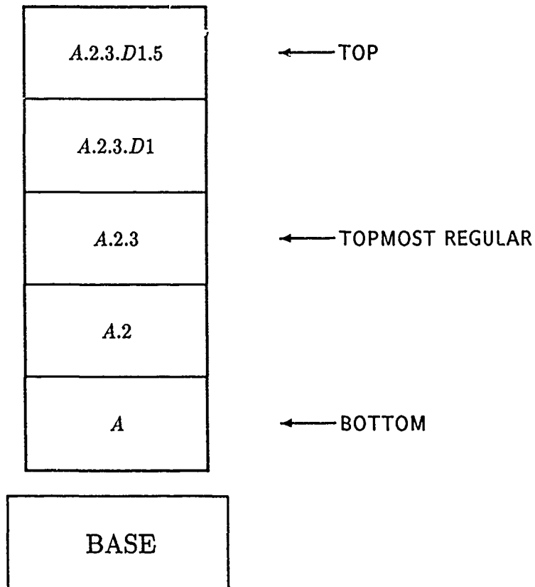
Figure 5-5: An example showing versions of an object to be prepared
