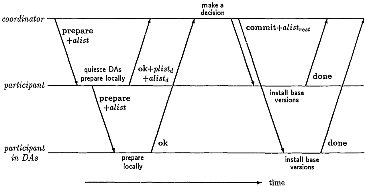
Figure 5-1: A time-space diagram of the modified Two Phase Commit protocol.
