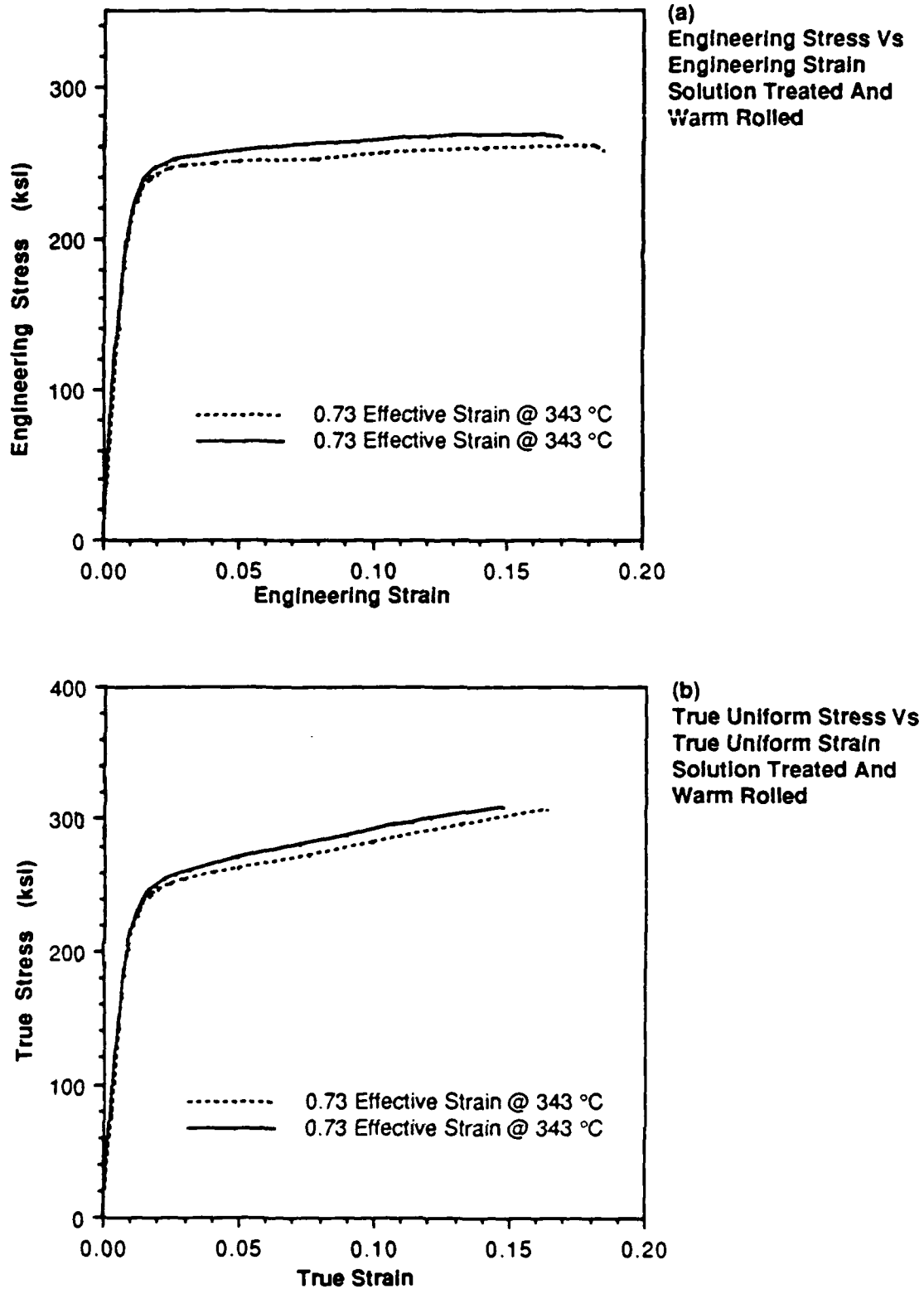
Fig. 17 (a,b) Engineering (a) and True Uniform (b) Stress-Strain Curves, Fe-12.5Mn-2.01Mo-1.15C Hadfield Steel, Warm Rolled 0.73 Effective Strain at 343 °C
