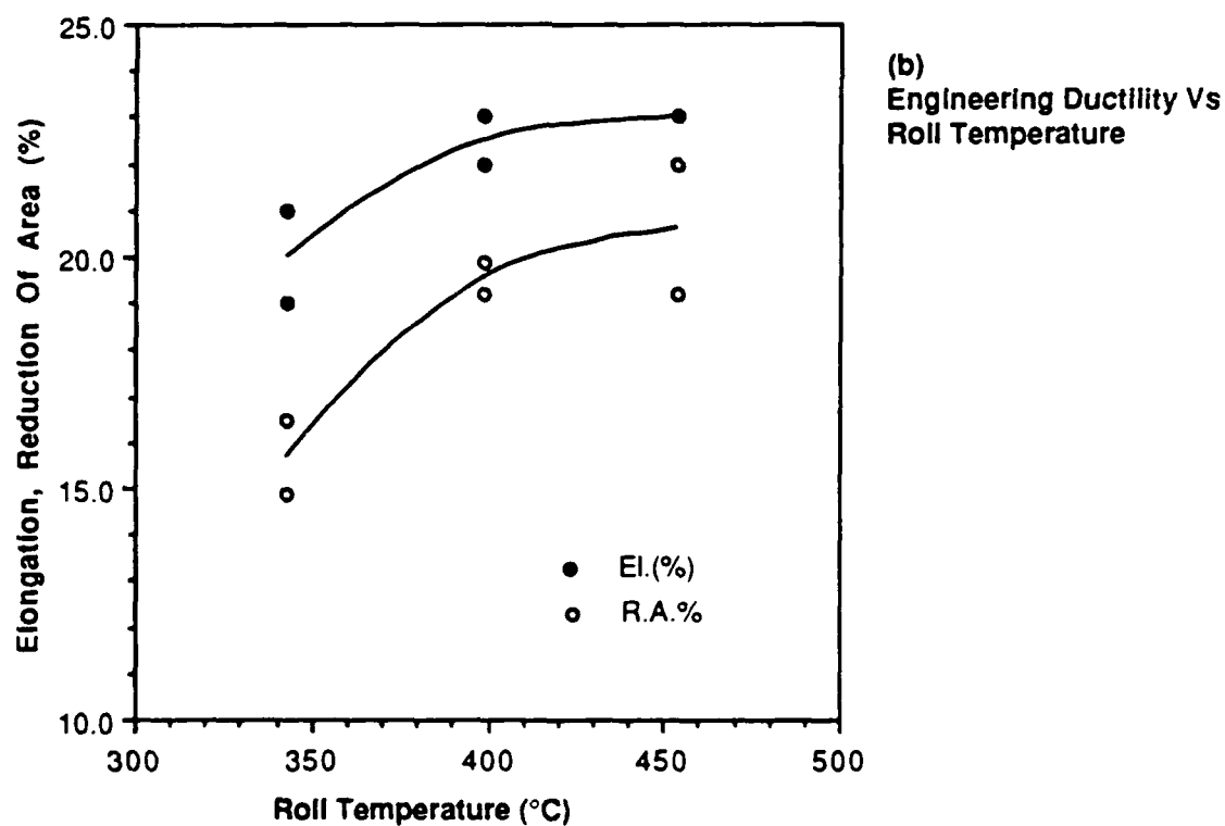
Fig. 29 (a-d) Trend Curves of Engineering Strength and Ductility in Tension Vs Roll Temperature at 0.70-0.75 Warm Roll Effective Strain
