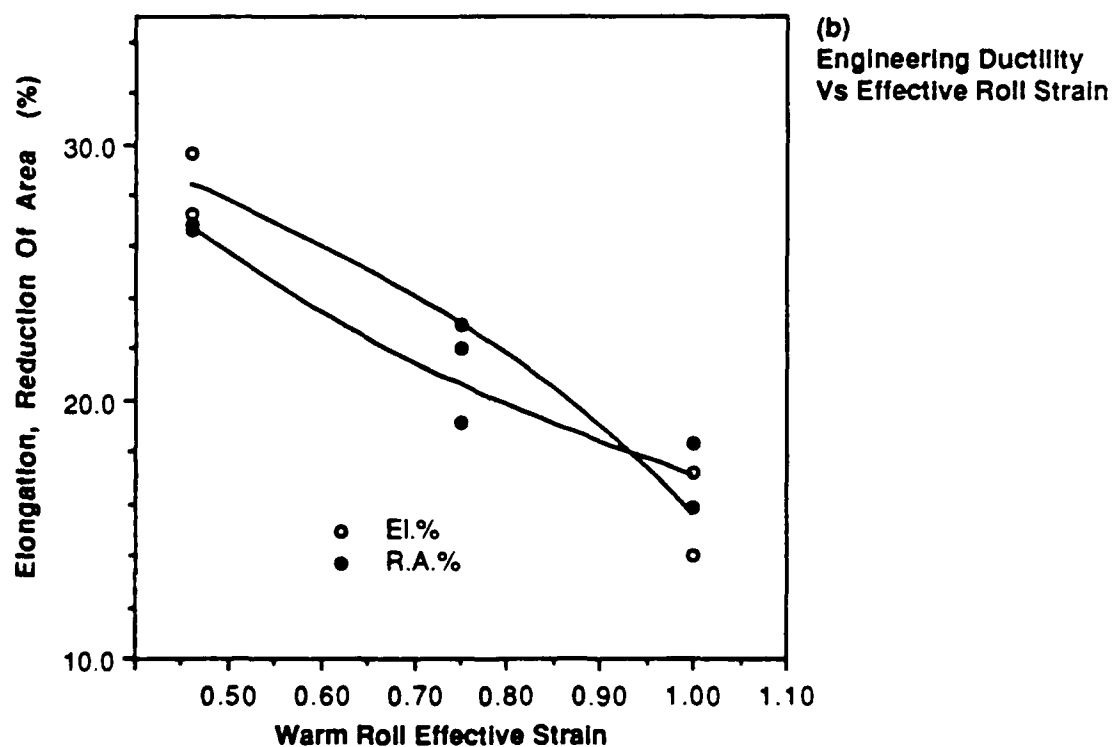
Fig. 30 (a-d) Trend Curves of Engineering Strength and Ductility In Tension Vs Warm Roll Effective Strain at 454 °C
