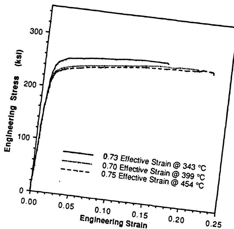
(a) Engineering Stress Vs Engineering Strain Solution Treated And Warm Rolled
