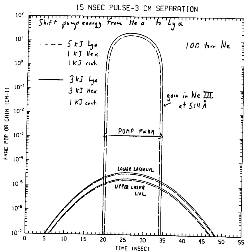
Fig. 2. Gain in the Ne III 514 \text{ \AA} laser transition, and population in the Ne III 1s^2 2s^2 2p^5 \text{ } ^5\text{S}_0 upper laser level and Ne III 1s^2 2s^2 2p^5 \text{ } ^3\text{P}_1 lower laser level are shown vs. time. The FWHM and assumed yields of the x-ray pump fluxes are indicated. Cold neon fill pressure is 100 torr.
