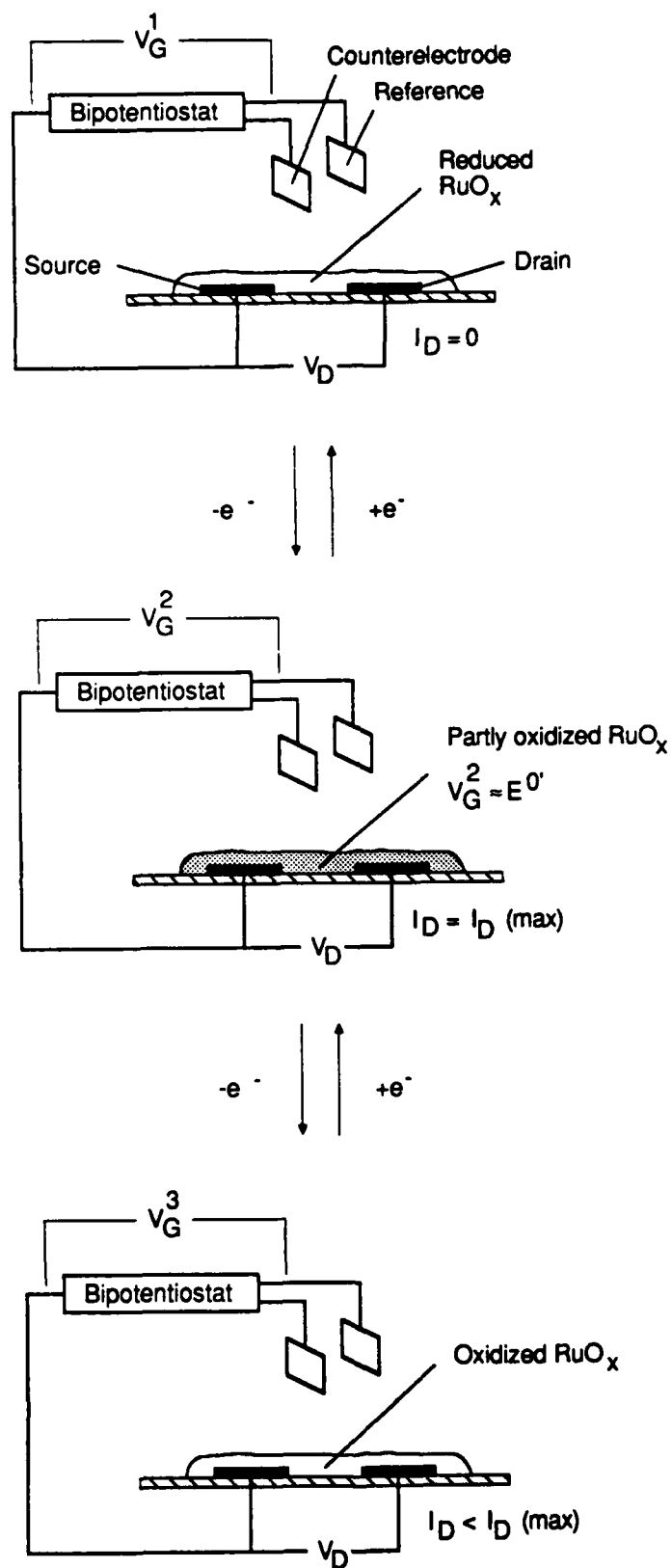
Scheme 1. \text{RuO}_x -based microelectrochemical transistor.
