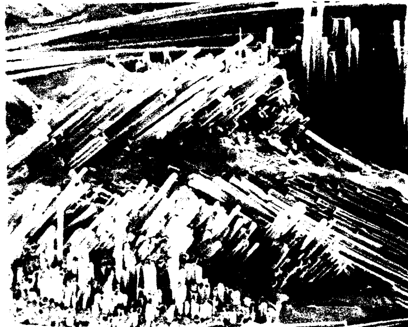
FRACTURE SURFACE OF CBN/CVI SiC MATRIX/CARBON COATED NICALON FIBER COMPOSITE [OXIDIZED 1000 °C, 70 hrs — RT = 11.2 ksi (77 MPa)]
