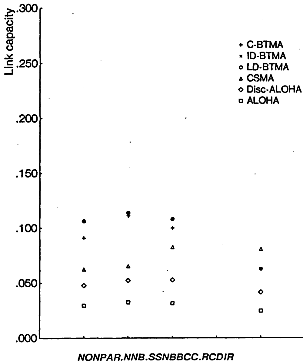
Fig. 9.36 Link capacity for nonparametric topologies with uniform nearest-neighbor traffic, for a spread spectrum system with bit-homogeneous receiver-directed codes, short bit duration, and a fourfold increase in transmitted power (see text for details)
