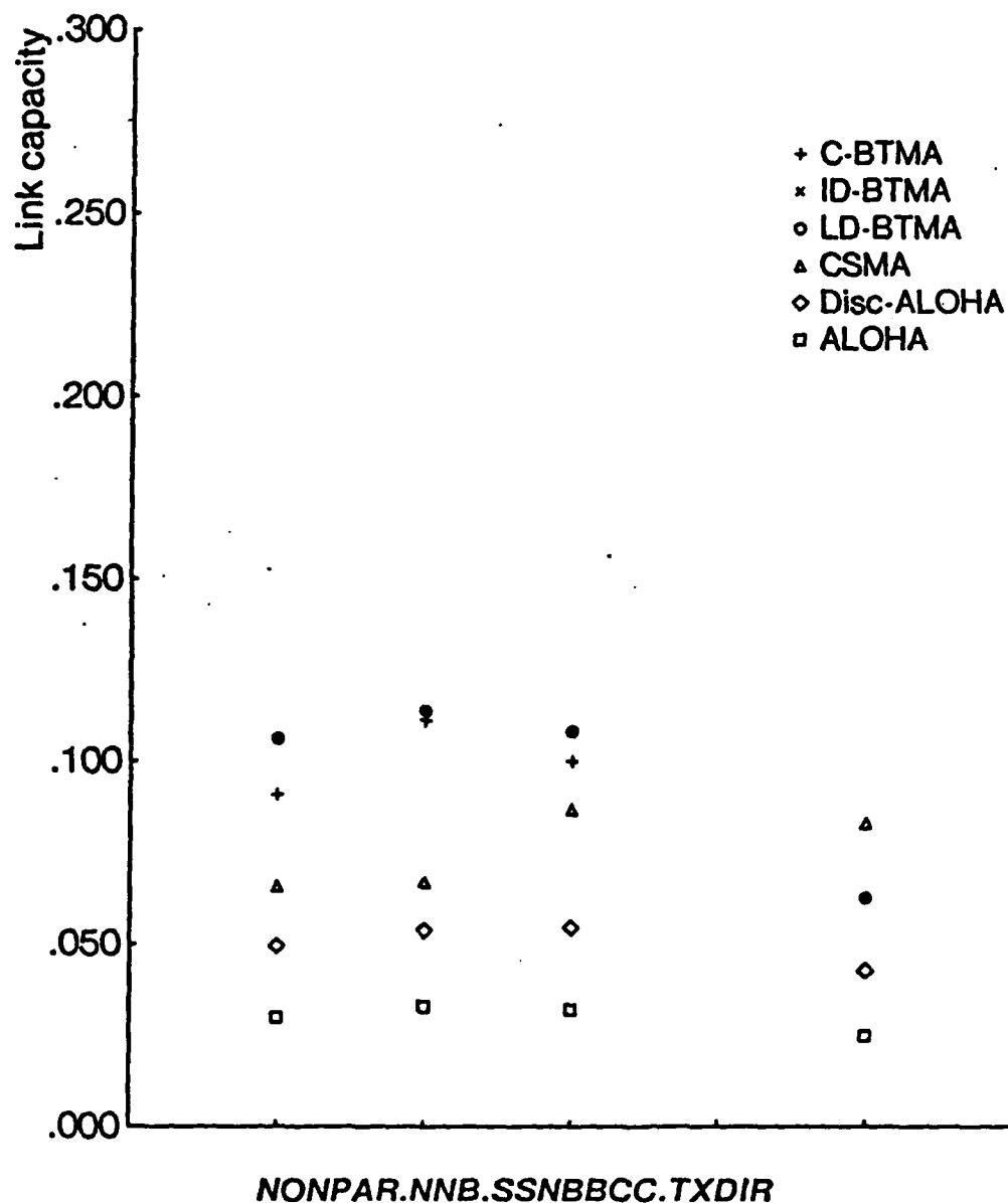
Fig. 9.35 Link capacity for nonparametric topologies with uniform nearest-neighbor traffic, for a spread spectrum system with bit-homogeneous transmitter-directed codes, short bit duration, and a fourfold increase in transmitted power (see text for details)
