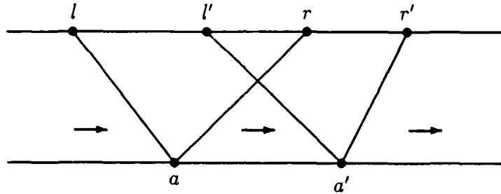
Figure 3: The dense cuts are checked by sweeping across the channel from one bottom to terminal to the next, maintaining a cone of dense cuts incident to the bottom terminal. At each stage, the algorithm keeps track of the maximum of the flows of all dense cuts seen so far.
