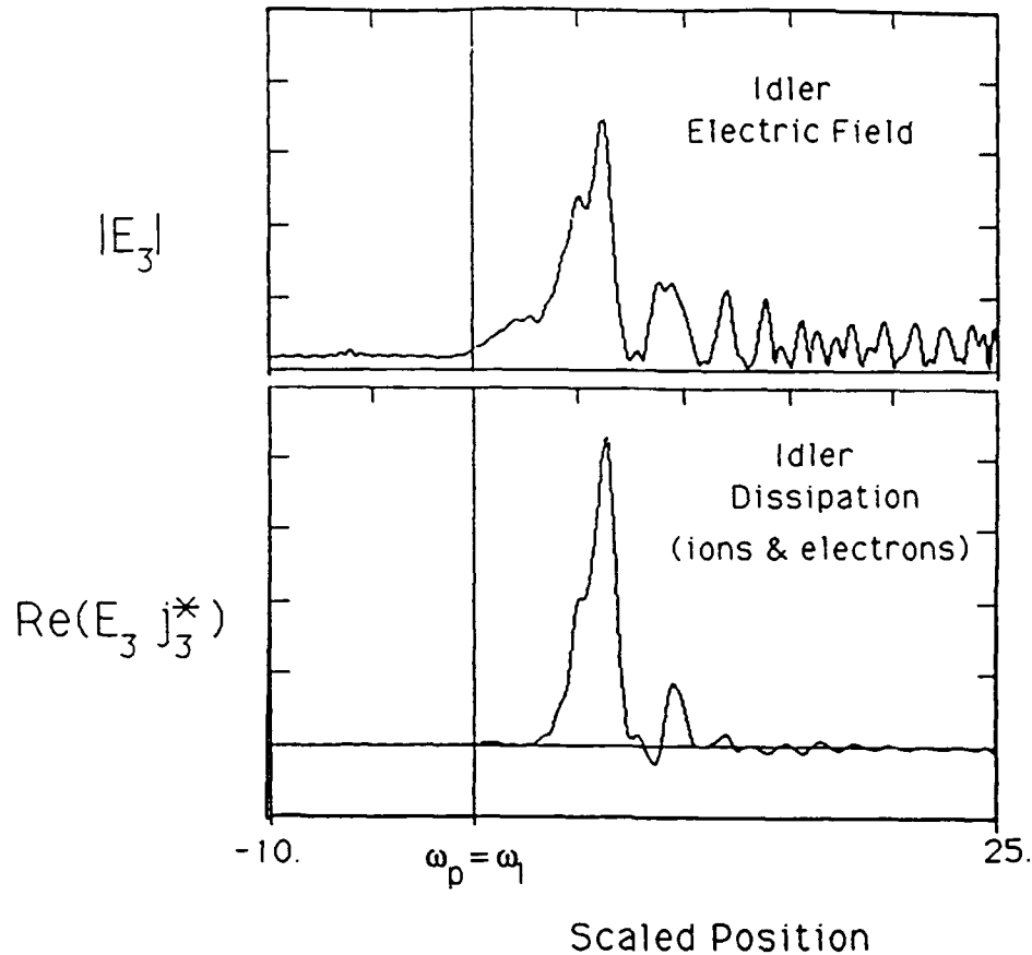
Figure 10. The idler field and spatial pattern of dissipation are shown for a frequency separation of 2% in the driving fields.
