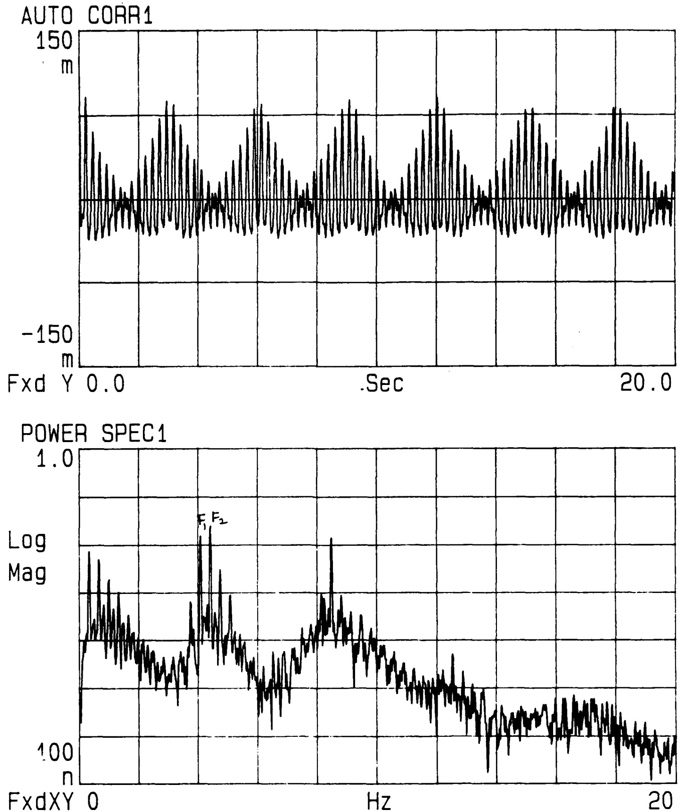
Figure 7 - Autocorrelation function and power spectrum for the quasiperiodic mixing layer
