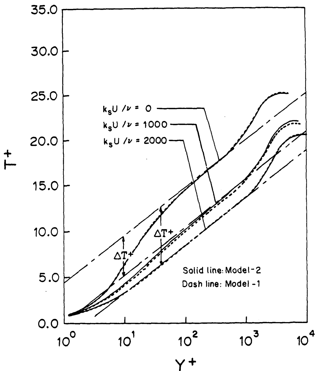
Figure 28. Temperature Profiles in Boundary Layers, Re_\tau = 5.10^6
