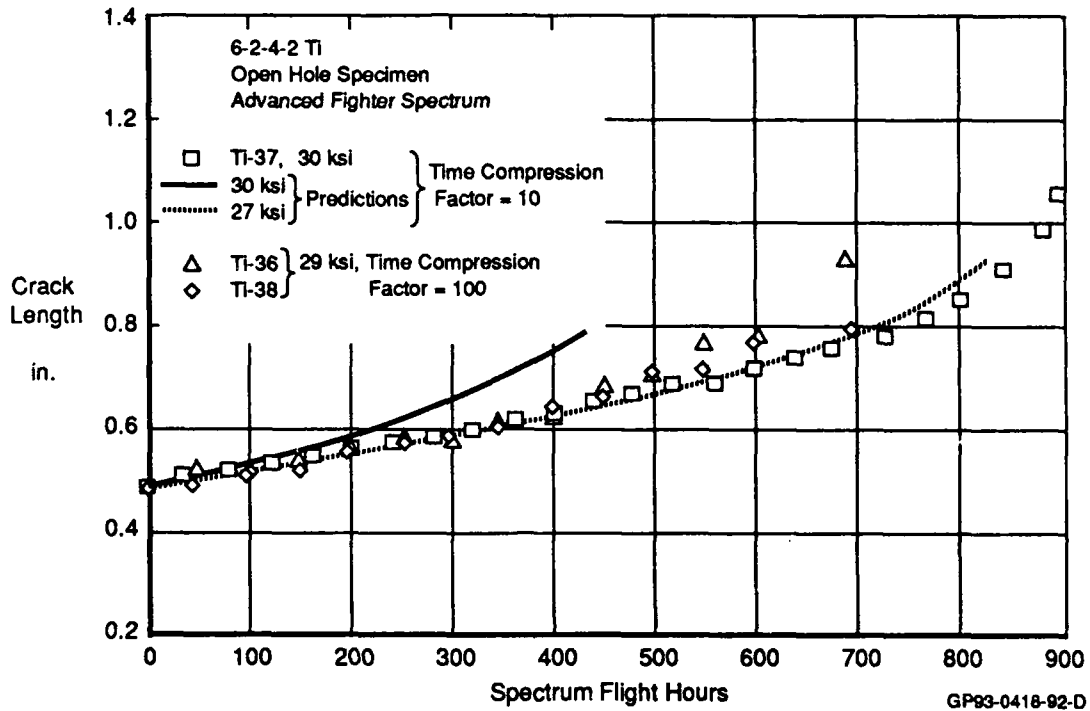
Figure 106. Verification Tests for 6-2-4-2 Ti Open Hole Specimens (Advanced Fighter Spectrum, Time Compression Factors = 10, 100)
