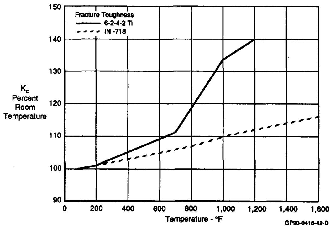
Figure 78. Fracture Toughness vs Temperature
