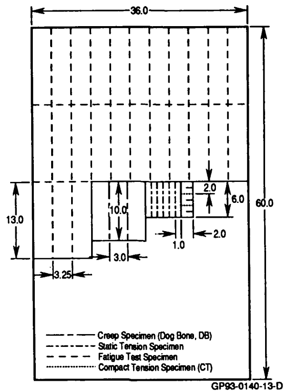
Figure 13. Specimen Layout
