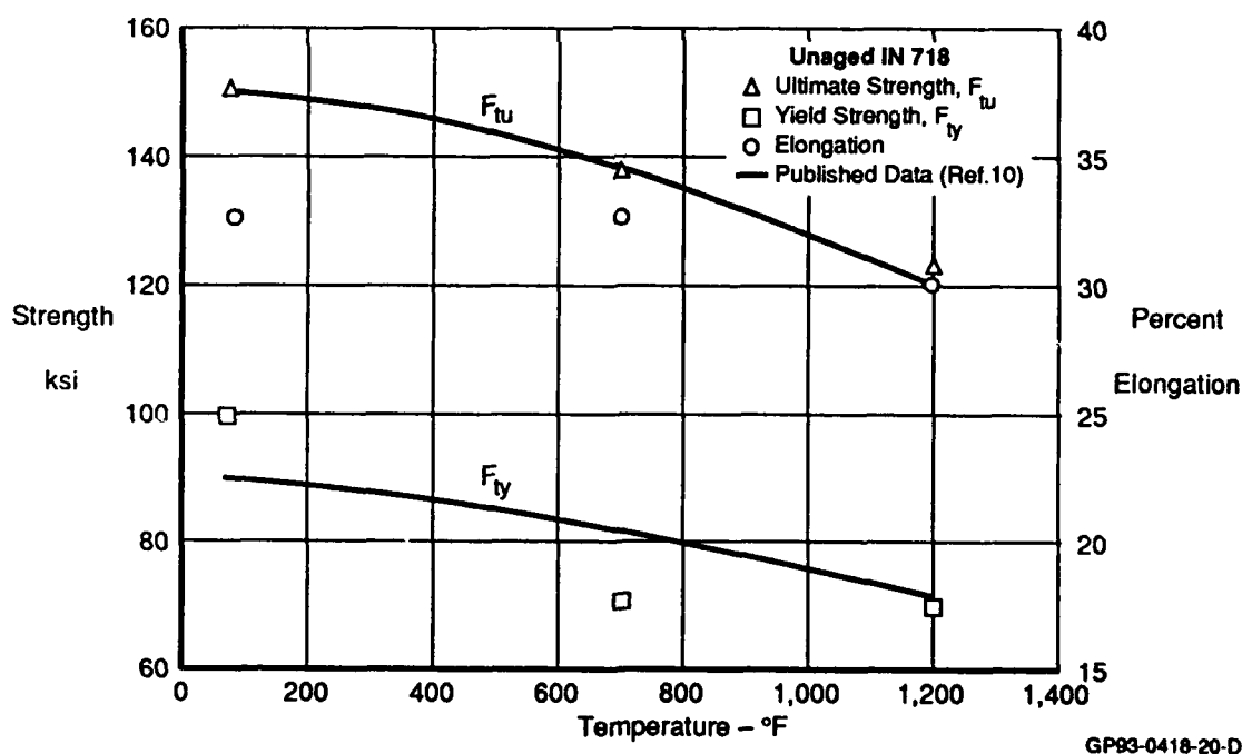
Figure 20. Static Tension Results of As-Received IN 718
