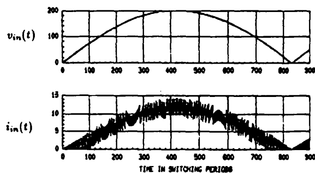
Figure 2: Current Loop
