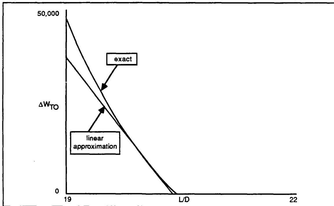
Figure D-7. Accuracy of Linear Approximation to Optimal Value of W_{TO}
