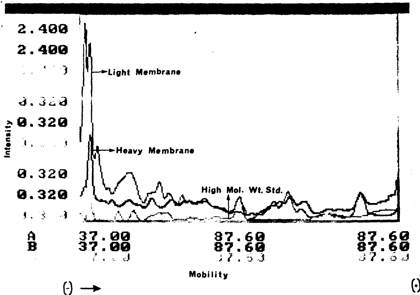
Fig.7 Scanning of SDS polyacrylamide electrophoresis gels on a LKB 2222-010 UltroScan XL Laser Densitometer.
