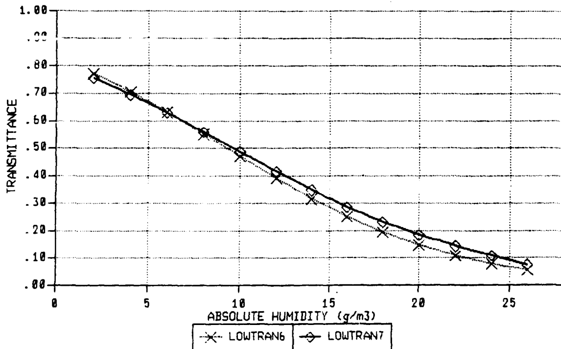
Figure 1. LOWTRAN6 and LOWTRAN7 Transmittance Vs Absolute Humidity, Rural Aerosol, 8-12 Micron Band.
