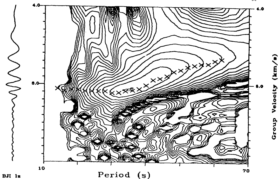
Figure 3 a. Dispersion of Rayleigh waves at BJI.
