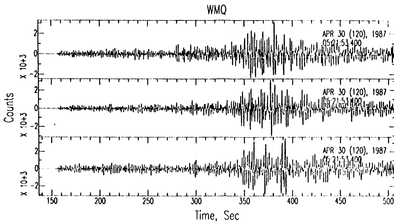
Figure 3.7 The event is near the Sino-Soviet border in southern Xinjiang (near the town of Wuqia). The is a shallow event. The seismograms in Fig. 3.9 are from the same region. They appear quite similar.
