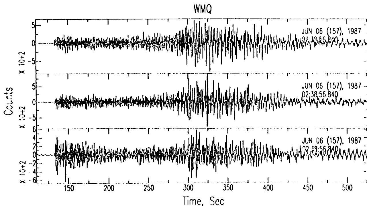
Figure 3.8 This is an Semipalatinsk event (evidently from the Degelen site, judging from the epicentral location and waveform - see more later). The L_g velocity for the first group is 3.4 km/sec. Compare Figure 3.10 and notice the overall difference between this figure and the Shagan River event records (Figure 3.10). ( P_n/L_g ) z for Shagan River events are consistently larger than those for the Degelen events. A characteristic large phase at about 15 seconds after the P_n is clearly observed in all cases for the Shagan River events, but not usually for the Degelen events. See next section for detailed comparison of P waves for these two groups of events. The short period ( \sim 5 seconds) surface waves train are very different for these events. But unfortunately the triggered records do not usually include the later waves.
