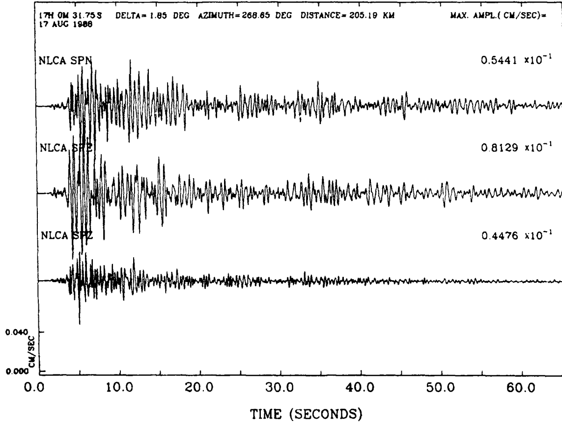
Figure 13. Sixty Seconds of the KEARSARGE Record at North Lake. Each trace represents pendulum motion, uncorrected for instrument response. Absolute amplitude scale (shown at bottom left) in cm/sec is used. Distance, azimuth, and back azimuth are given at the top.
