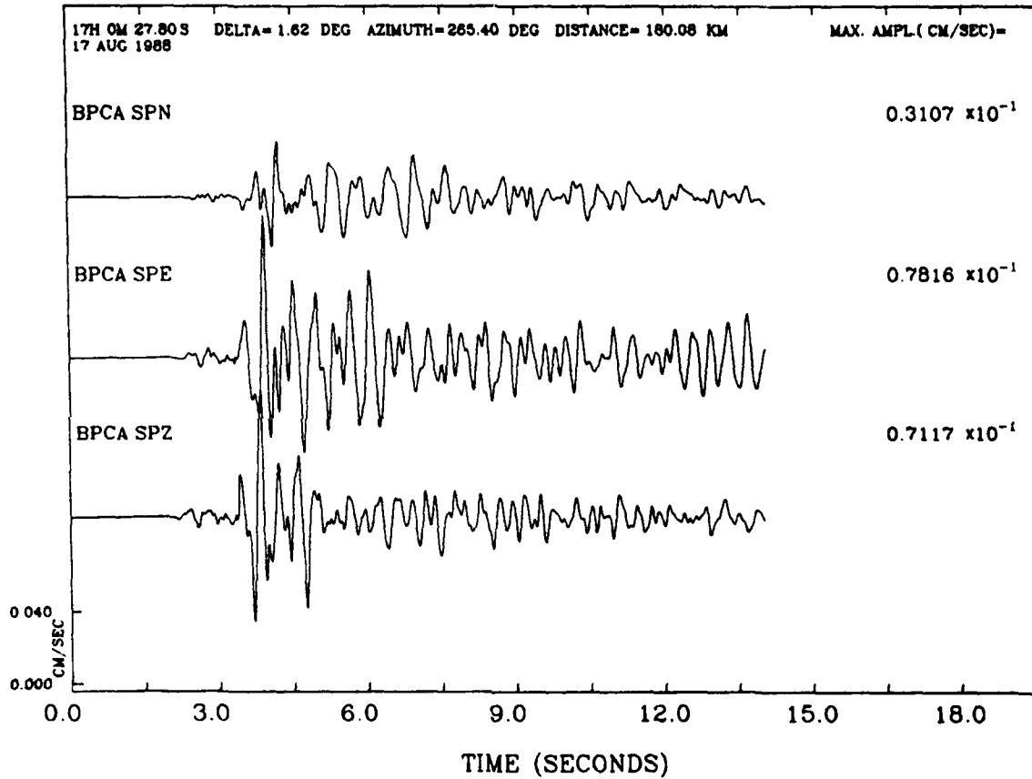
Figure 7. Seismograms of KEARSARGE Test Recorded at Big Pine, California. Each trace represents pendulum motion, uncorrected for instrument response. Absolute amplitude scale (shown at bottom left) in cm/sec is used. Distance, azimuth, and back azimuth are given at the top.
