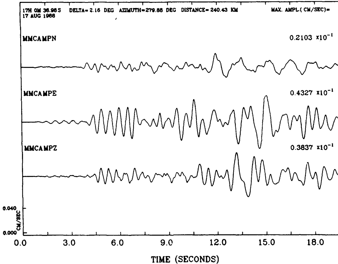
Figure 3. Seismograms of KEARSARGE Test Recorded at Mammoth Lakes, California. Each trace represents pendulum motion, uncorrected for instrument response. Absolute amplitude scale (shown at bottom left) in cm/sec is used. Distance, azimuth, and back azimuth are given at the top.
