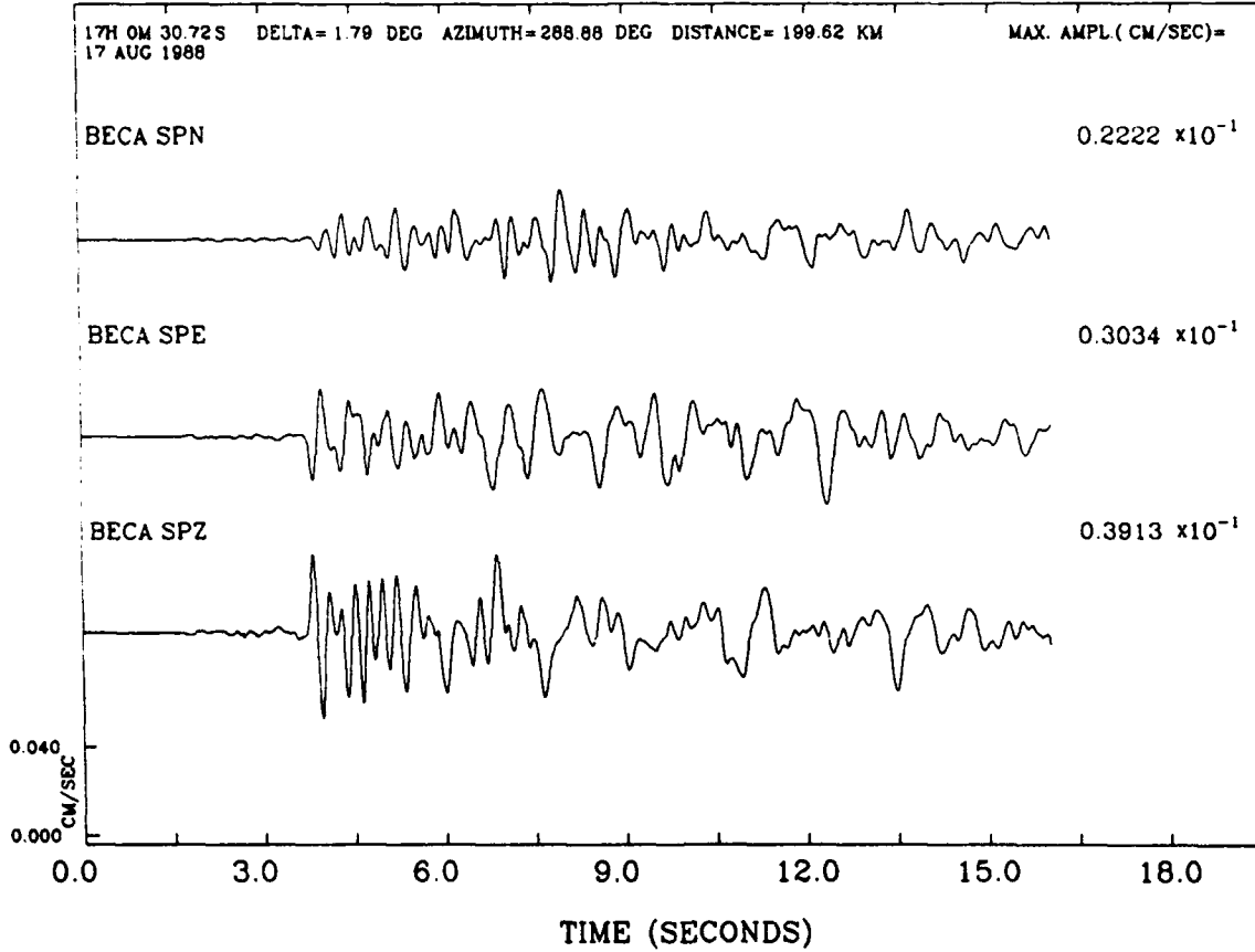
Figure 2. Seismograms of the Pn and Pg Phases From the KEARSARGE Test Recorded at Benton, California. Each trace represents pendulum motion, uncorrected for instrument response. Absolute amplitude scale (shown at bottom left) in cm/sec is used. Distance, azimuth, and back azimuth are given at the top.
