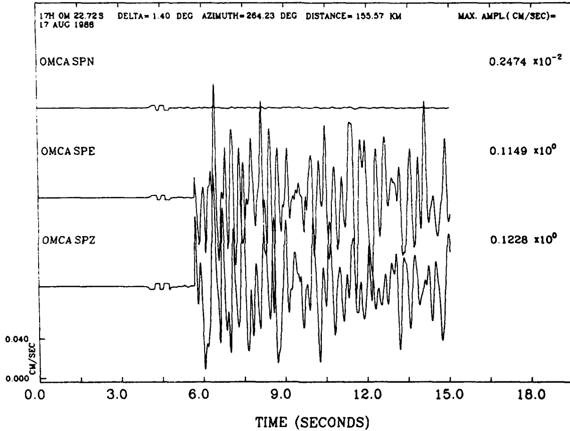
Figure 4. Seismograms of KEARSARGE Test Recorded at Overholtz Mine, California. Each trace represents pendulum motion, uncorrected for instrument response. Absolute amplitude scale (shown at bottom left) in cm/sec is used. Distance, azimuth, and back azimuth are given at the top.
