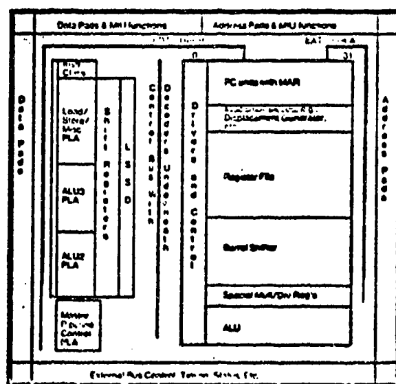
Figure 2: MIPS Floorplan
