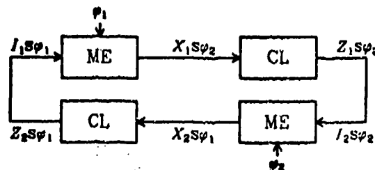
Figure 4. A typical two-phase finite state machine show the syntax and consistency of the clocking types and composition rules.
