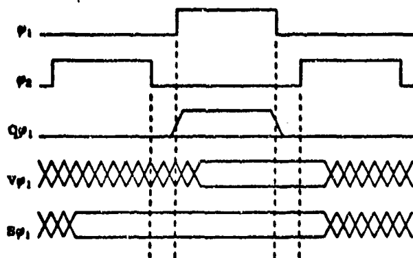
Figure 2. Some representative clocking types, showing the sequence of events. Q, v, and s stand for qualified, valid, and stable.
