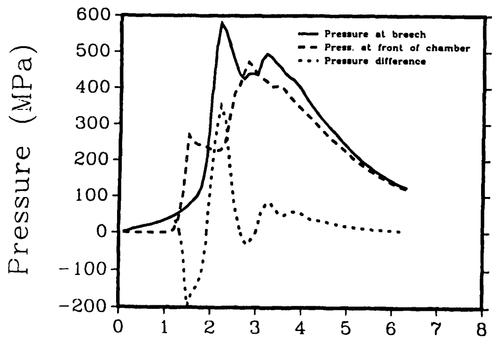
Figure 9. Predicted Pressure Profiles - Base Ignition, Forward Ullage, and Grain Fracture
