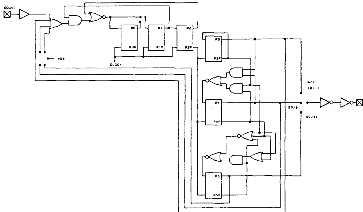
Fig. 2.1-1 Mask programmable prescaler.
