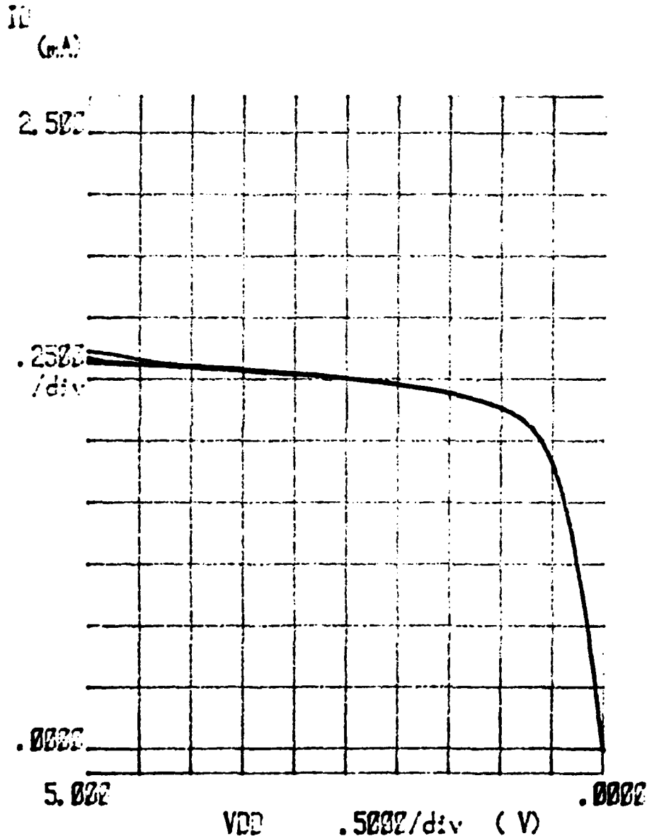
Fig. 4.2.2-10 Basic pull-up transfer curves with biased backgating finger 27\text{ }\mu\text{m} from drain.
