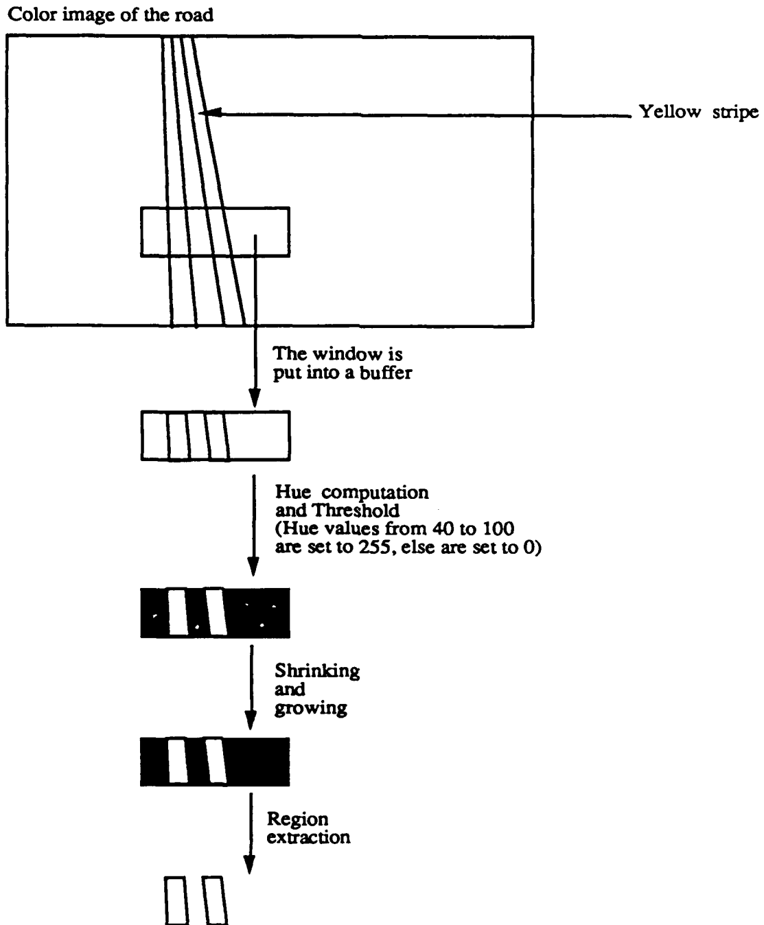
Figure 9: Yellow stripe extraction scheme
