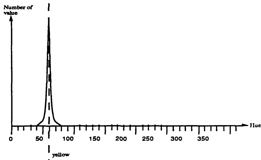
Figure 7: Histogram of the hue value for yellow lines without shadows in a sequence of images (camera sony model DXC-3000. Lens Fujinon-TV.Z). The values are symmetrically distributed around 60^\circ with a variation of 20^\circ on either side.
