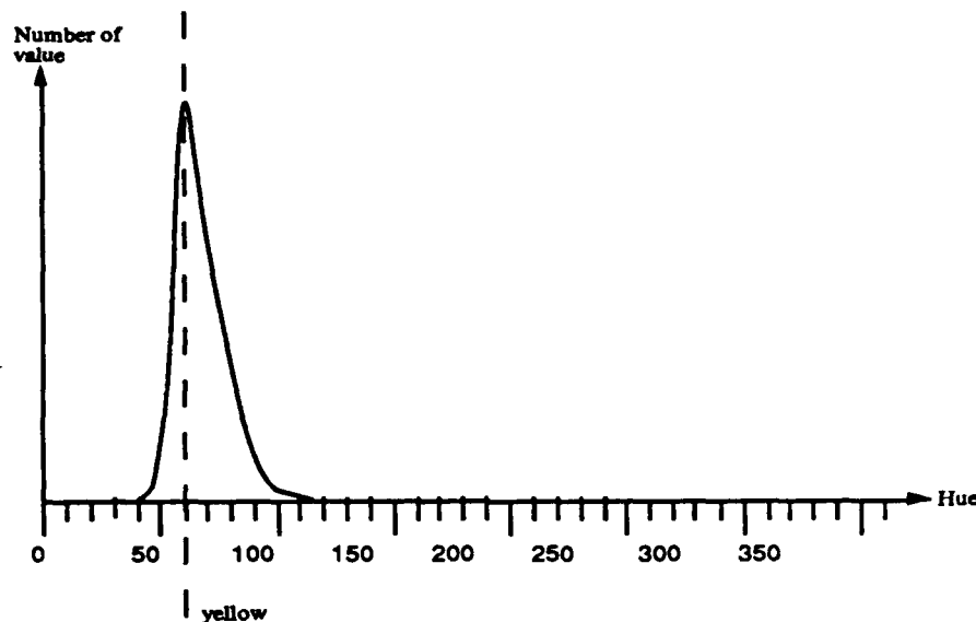
Figure 8: Histogram of the hue value for yellow lines with shadows in a sequence of images (camera sony model DXC-3000. Lens Fujinon-TV.Z). The values are no longer symmetrically distributed around 60°, but slightly skewed instead. The values lie between 40° and 120°, but there are very few values from 100° to 120°.
