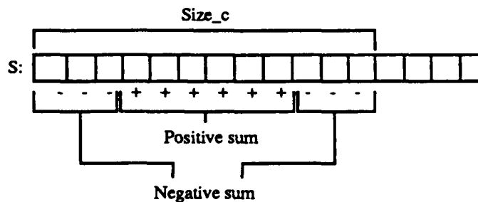
figure 3: Computation of the first correlation
