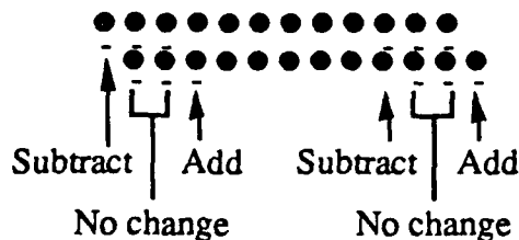
figure 5: Computation of the new negative sum
