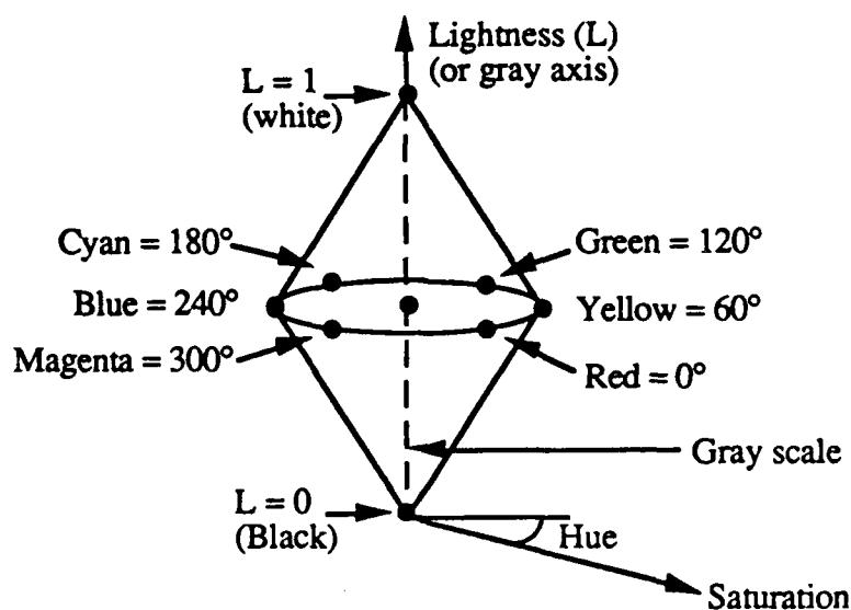
Figure 6: The HLS color model
