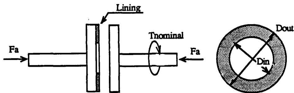
Figure 2-7: Clutch Example
