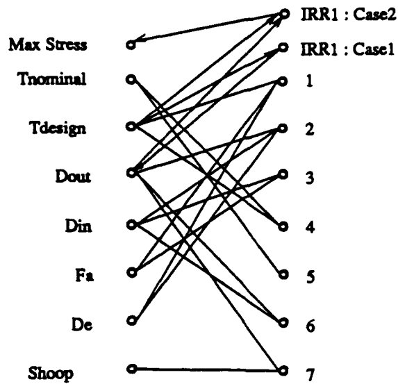
Figure 2-16: A Directed Bipartite Graph representation
