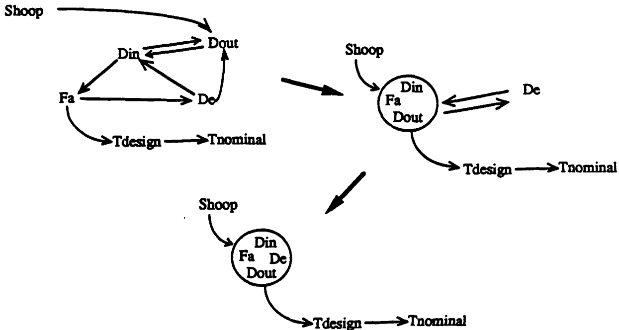
Figure 2-13: Finding strong components in a bi-partite graph.
