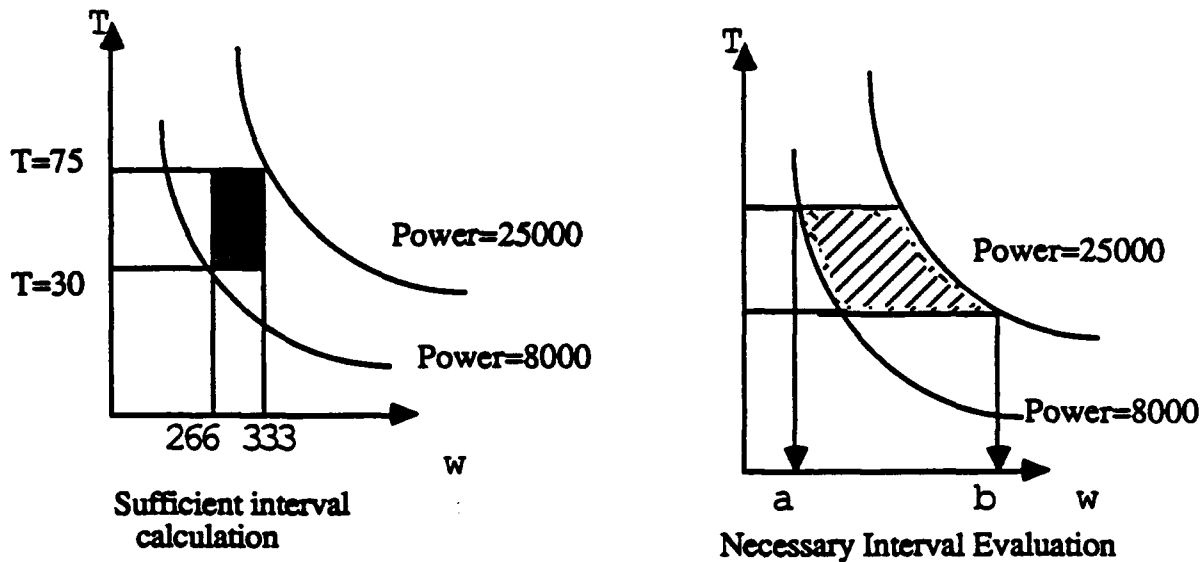
Figure 1-4: Constant Power Curves for a D.C. Motor
