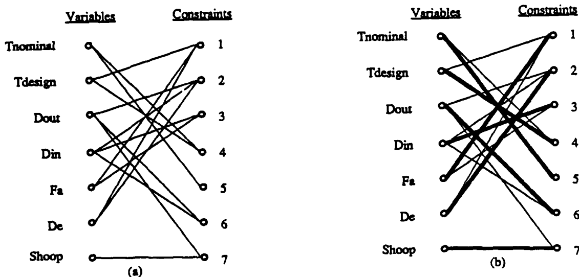
Figure 2-11: Bipartite Matching
