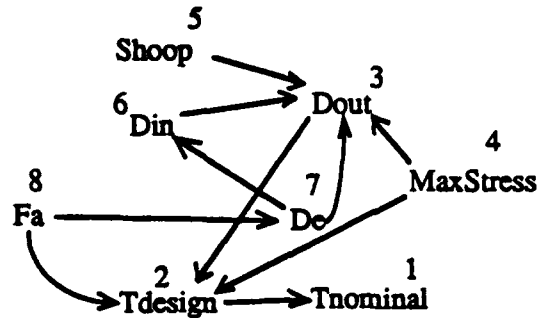
Figure 2-18: Dependency Graph with Unidirectional Constraints
