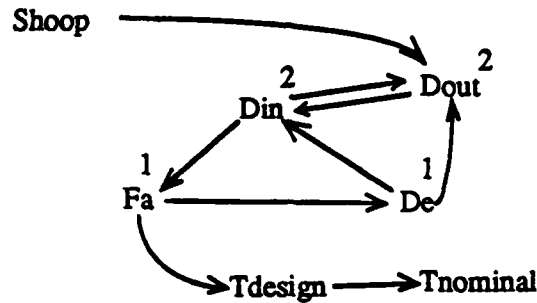
Figure 2-15: Counting the number of dependents at each node.
