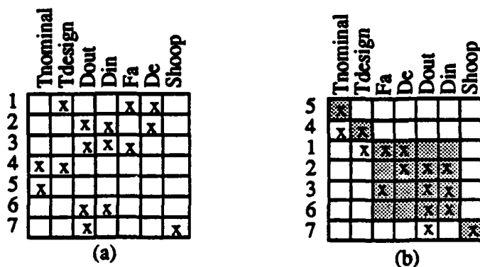
Figure 2-9: Adjacency Matrix Representation of the Ordering Task
